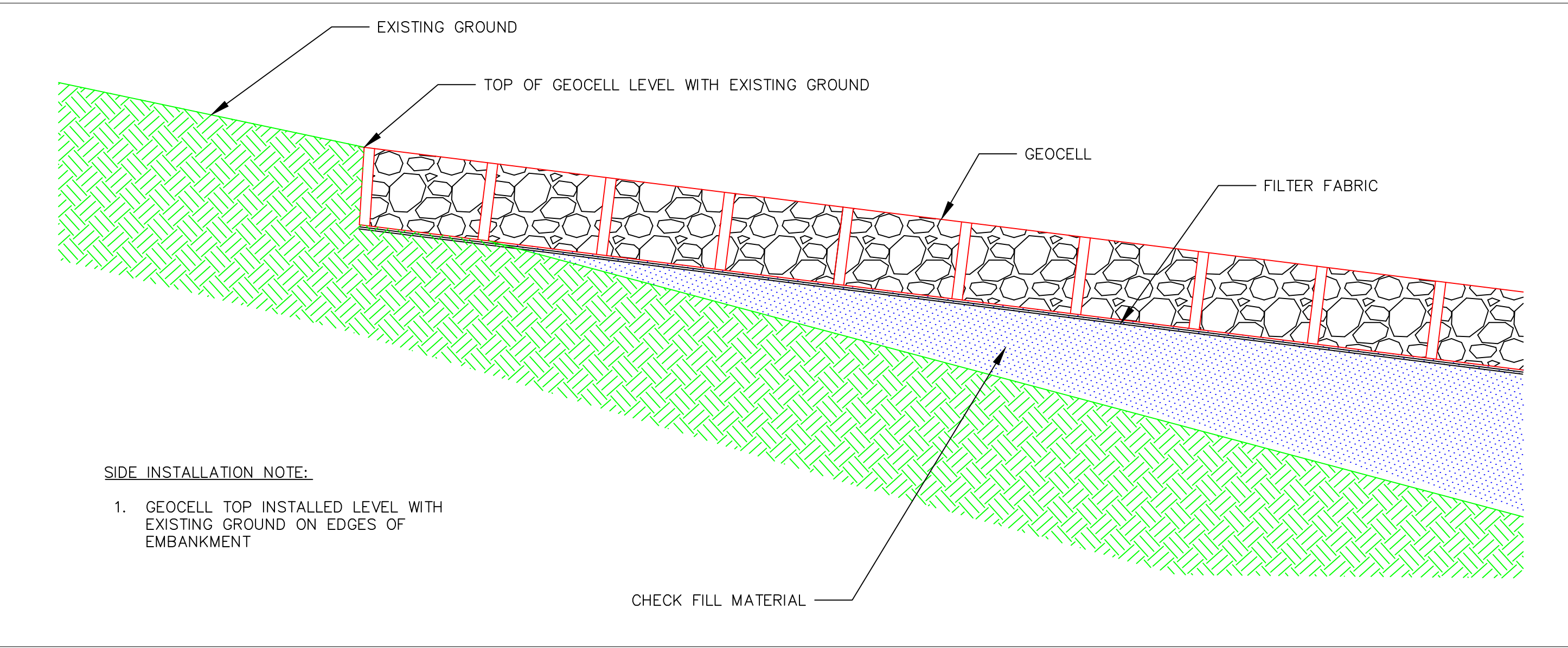
GEOCELL SIDE INSTALLATION DETAIL NOT TO SCALE
