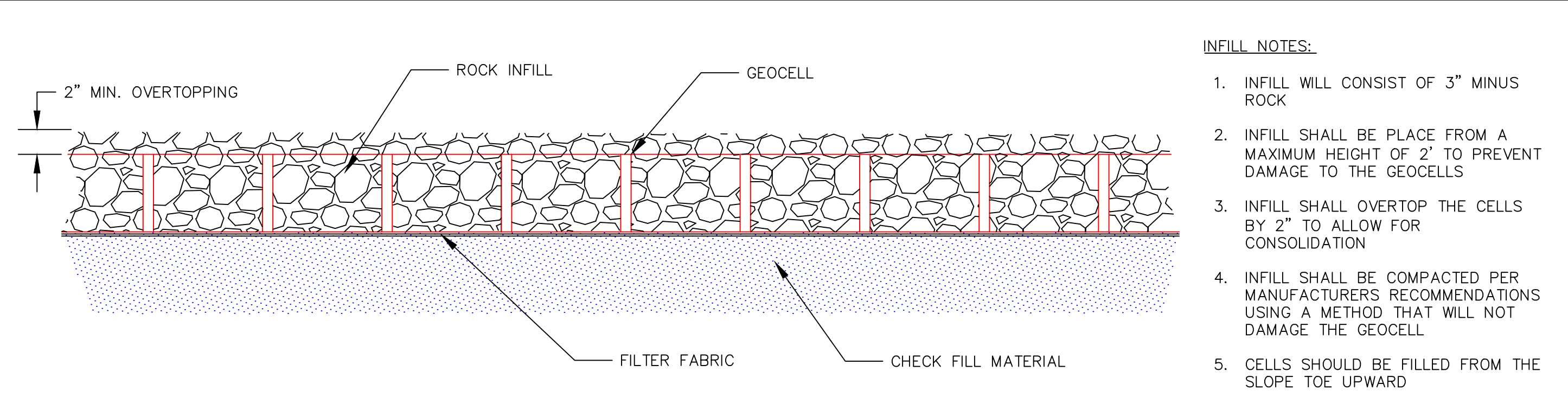
GEOCELL INFILL DETAIL NOT TO SCALE
