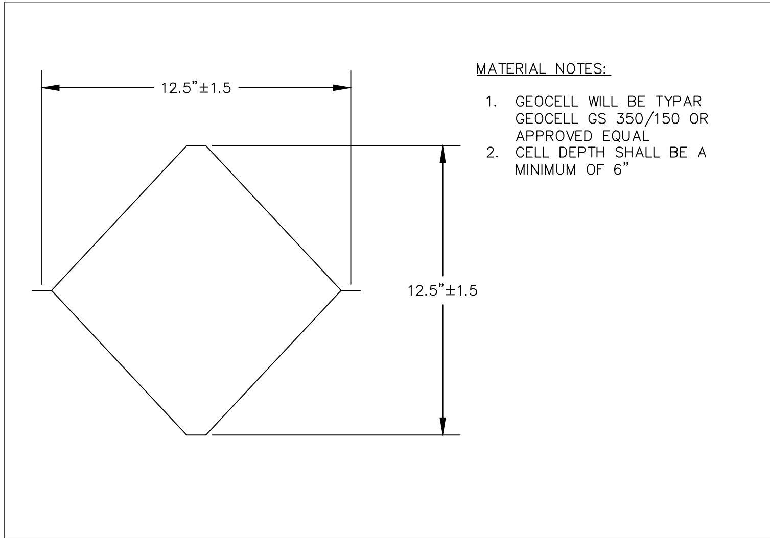
GEOCELL DIMENSION DETAIL NOT TO SCALE
