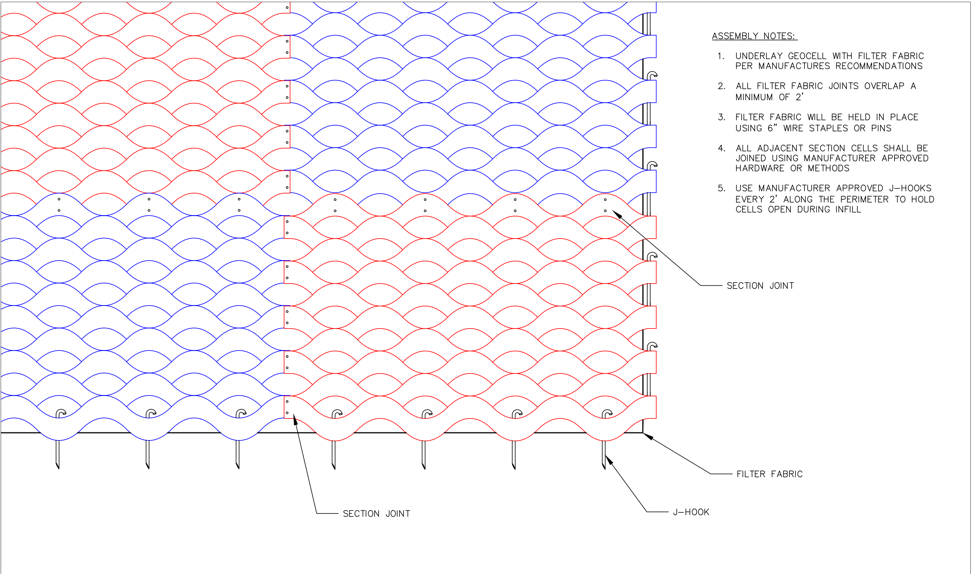
GEOCELL ASSEMBLY DETAIL NOT TO SCALE
