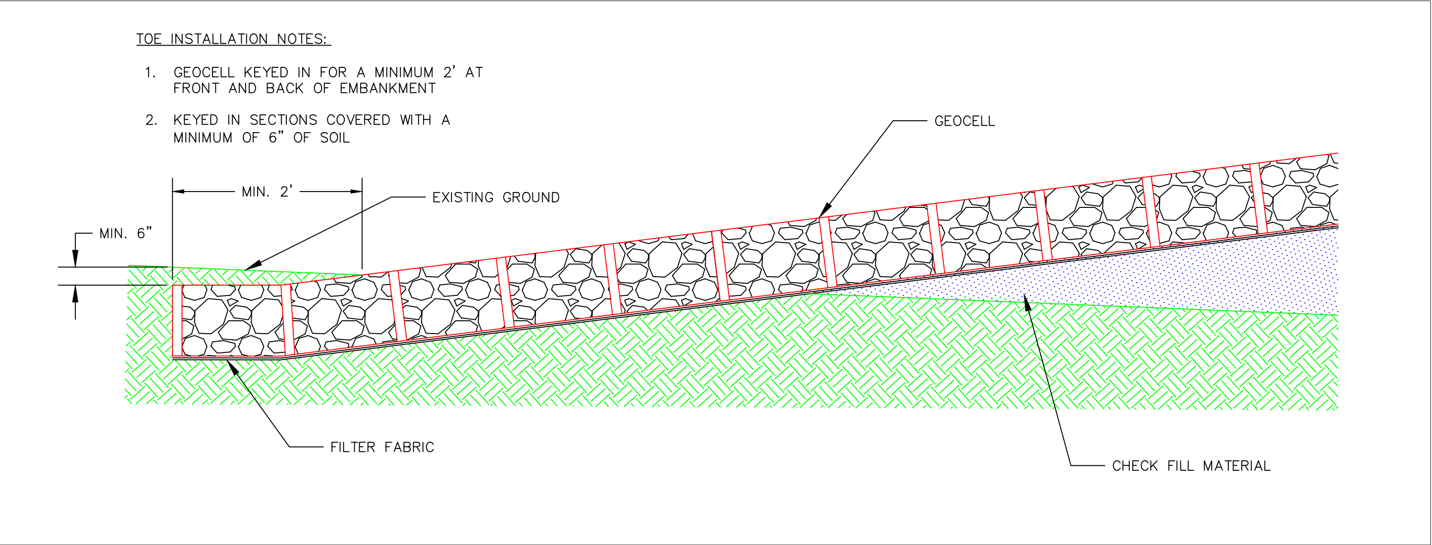
GEOCELL TOE INSTALLATION DETAIL NOT TO SCALE
