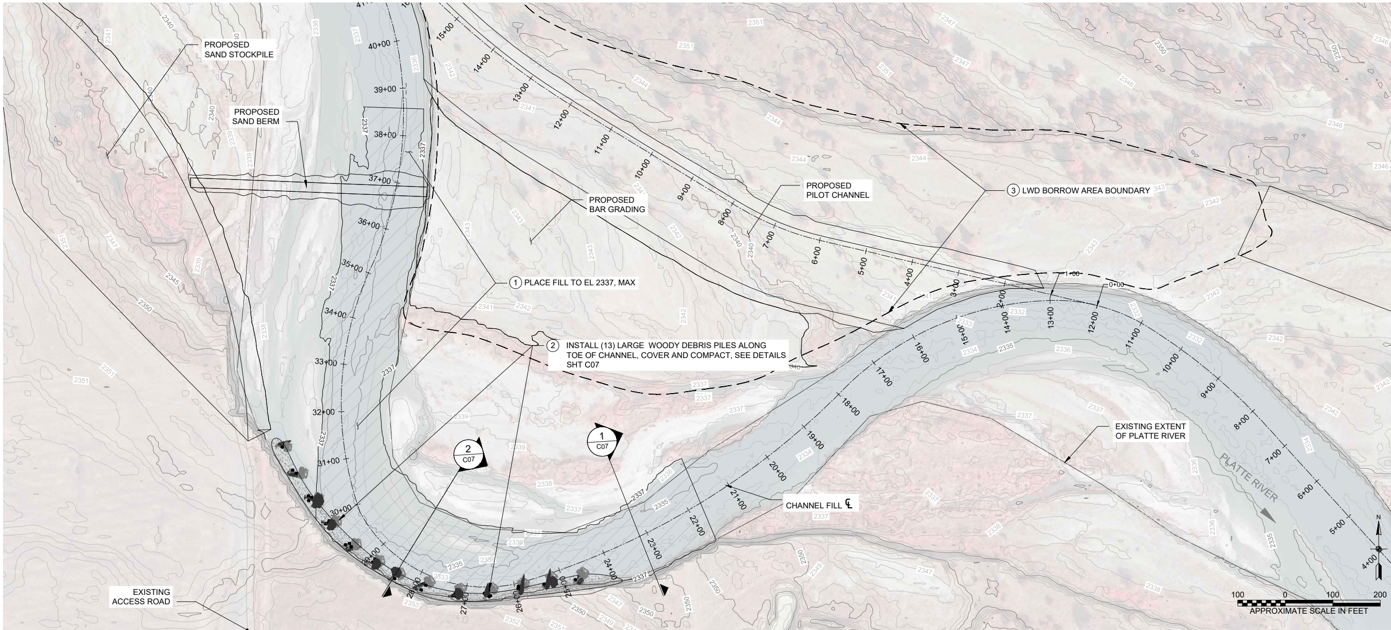
CHANNEL FILL - PLAN
