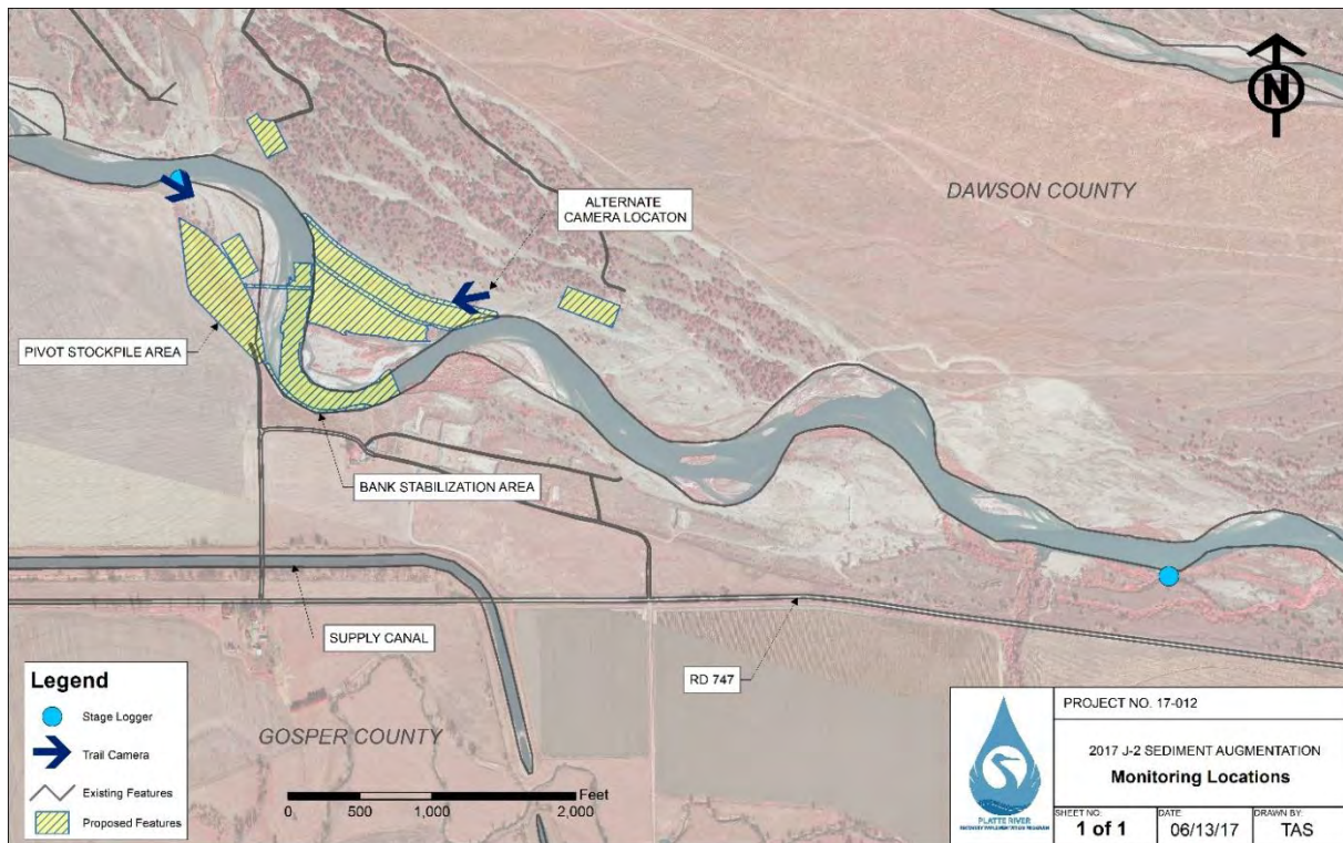
Figure 2. Proposed monitoring locations and areas to be graded.
