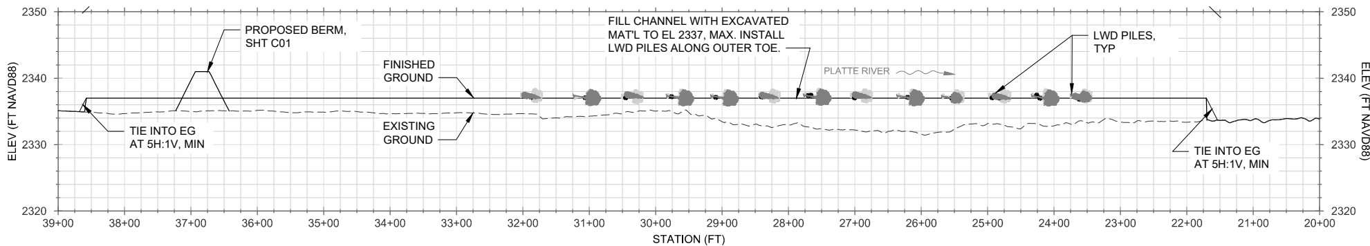
CHANNEL FILL - PROFILE
