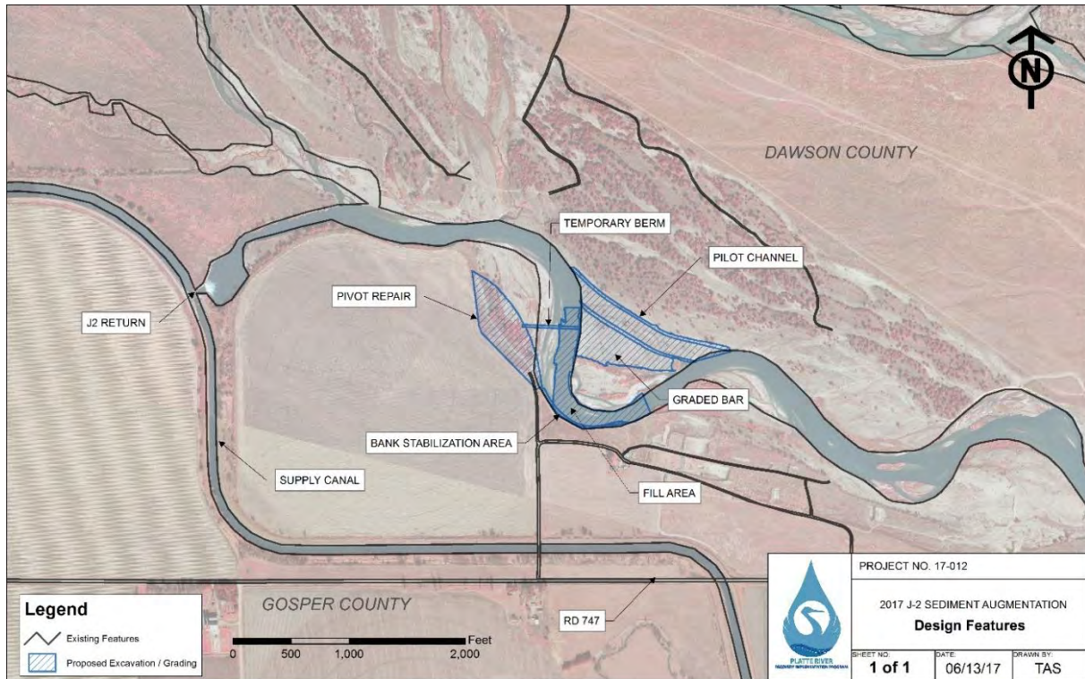
Figure 1. Overview of Sediment Augmentation Design, illustrating J2 return and proposed grading areas.
