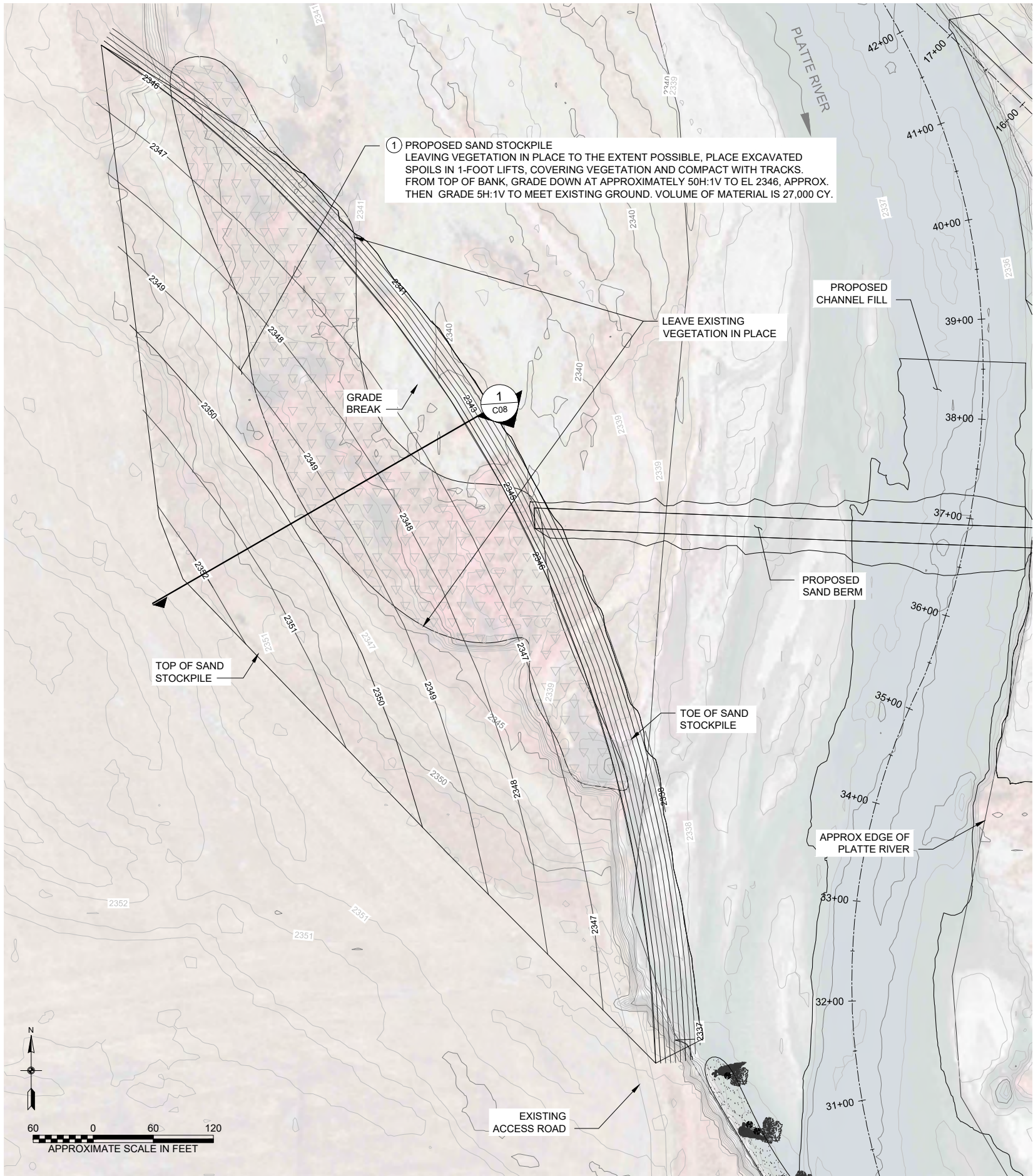
SAND STOCKPILE PLAN
