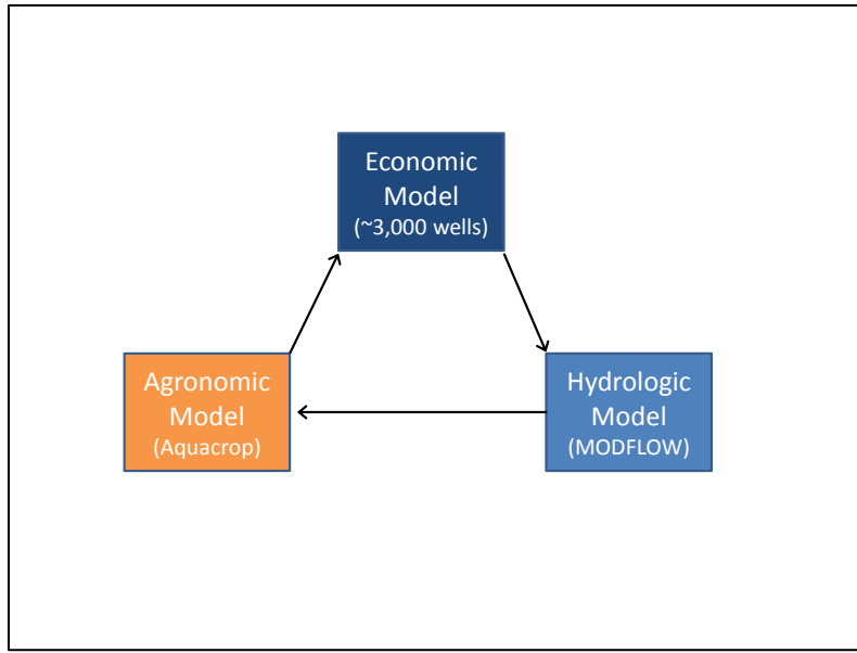
Figure 3: Basic structure of model framework used to evaluate groundwater management policies
