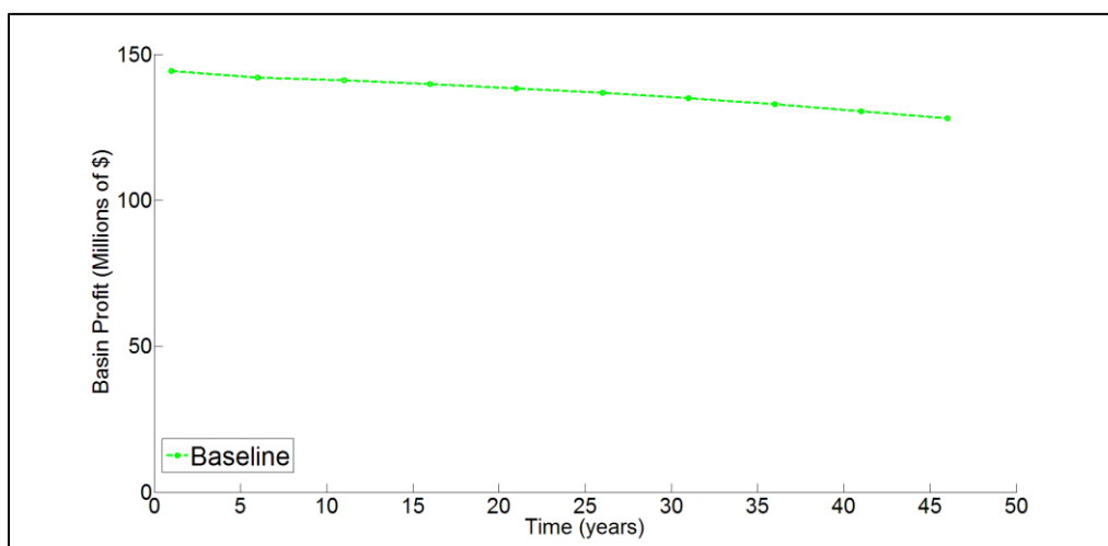
Figure 16: Average baseline profits in the Basin over 50 years (5-year averages)
