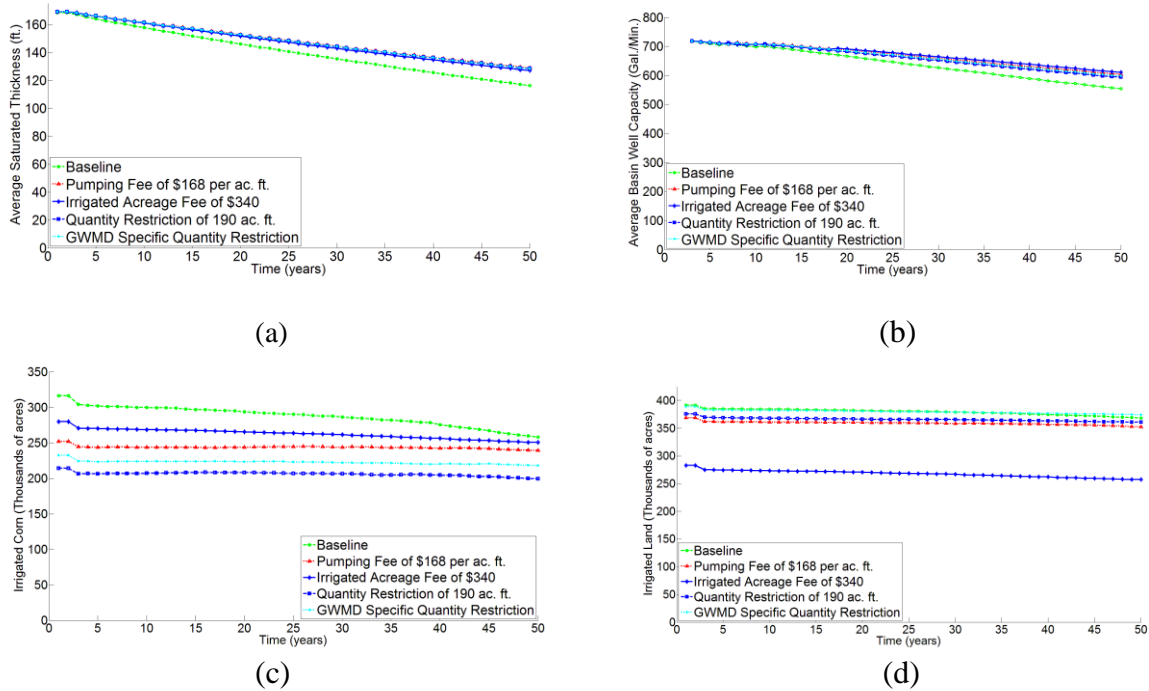
Figure 18: Examining Basin-wide impacts of water management policies. Panel (a) presents average saturated thickness over time, panel (b) presents average well capacity over time, panel (c) presents acres of irrigated corn, and panel (d) presents total acres of irrigated land.
