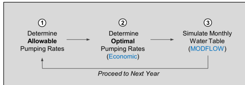
Figure 10. Flow chart of hydro-economic modeling process.
