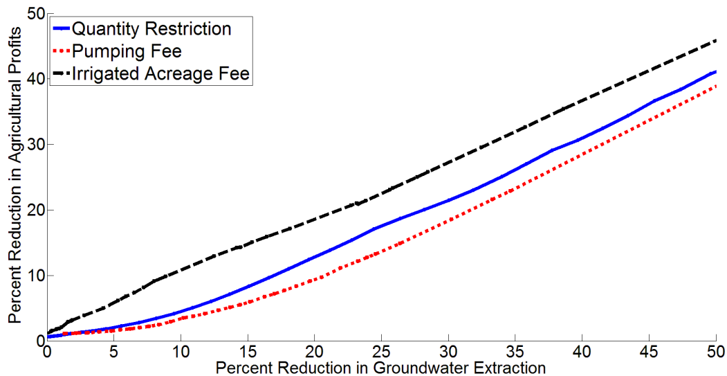
Figure 13: Comparison of relationship between reduction in groundwater use and decrease in producer profit for various management policies.
