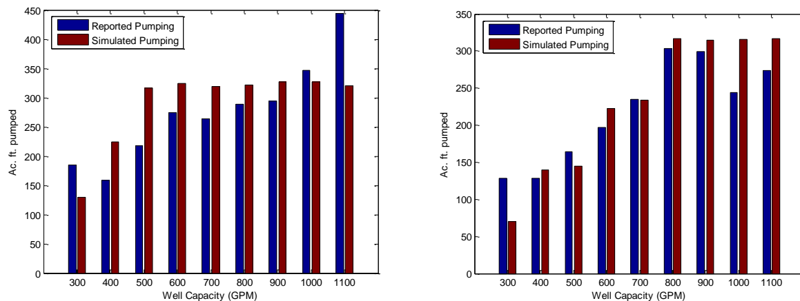
Figure 12: Comparison of observed and modeled pumping for sandy soil in the north (left panel) and south (right panel) in a low recharge year.
