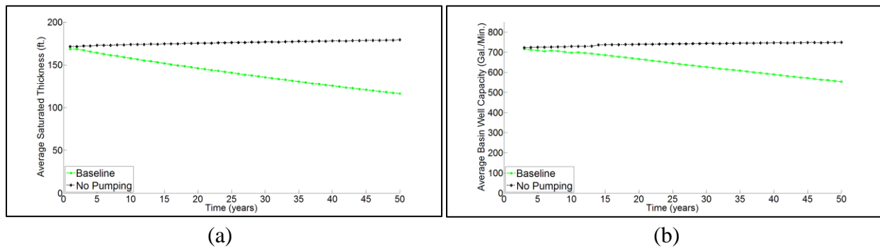
Figure 15: Basin-wide average saturated thickness (panel (a)) and well capacity (panel (b)) predicted by MODFLOW under baseline and no agricultural pumping scenarios.
