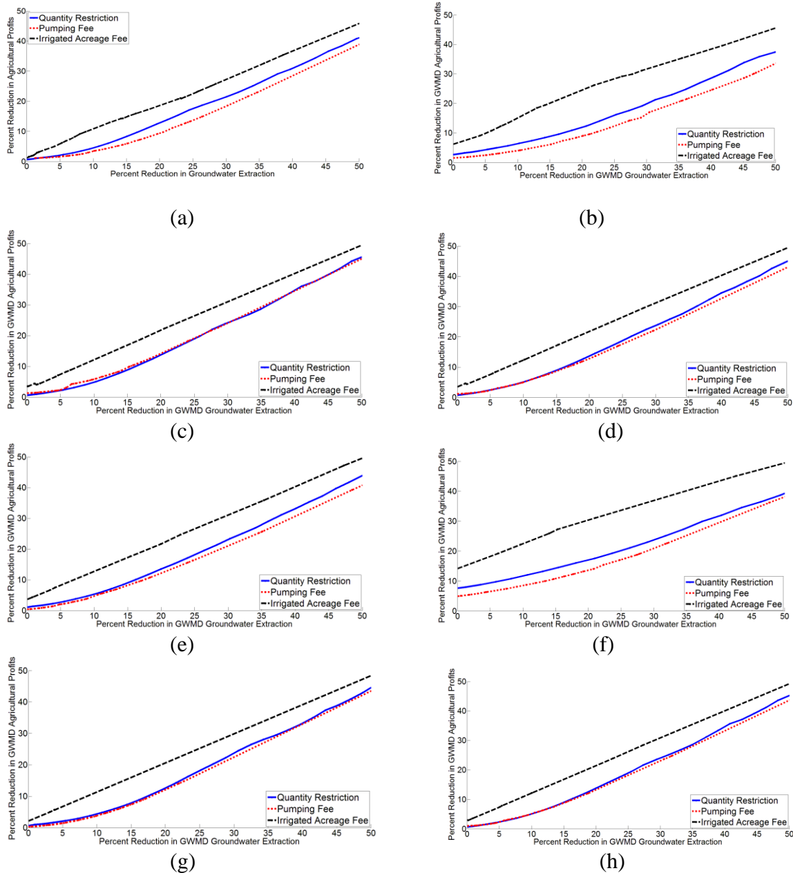
Figure 14: Comparison of relationship between reduction in groundwater use and decrease in producer profit by GWMD associated with uniform Basin-wide policies – (a) Basin-wide, (b) Arikaree, (c) Central Yuma, (d) Frenchman, (e) Marks Butte, (f) Plains, (g) Sand Hills, (h) W-Y.
