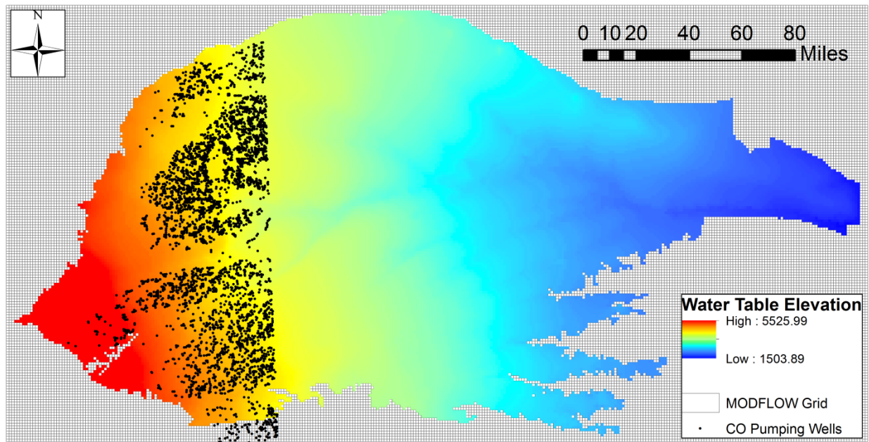
Figure 8. Example simulated output (water table elevation in feet) from the MODFLOW model.
