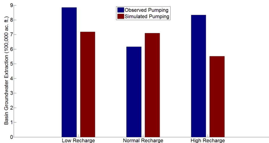
Figure 11. Comparison of modeled and reported groundwater use for three years of recharge realizations.
