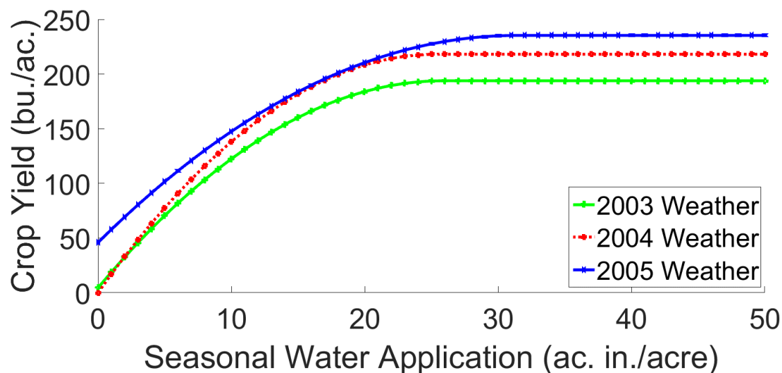
Figure 6: Example of water-yield relationship for corn in 2003,2004 and 2005, given that 130 acres are planted on silty soil in the northern climatic zone with a well capacity of 700 GPM.
