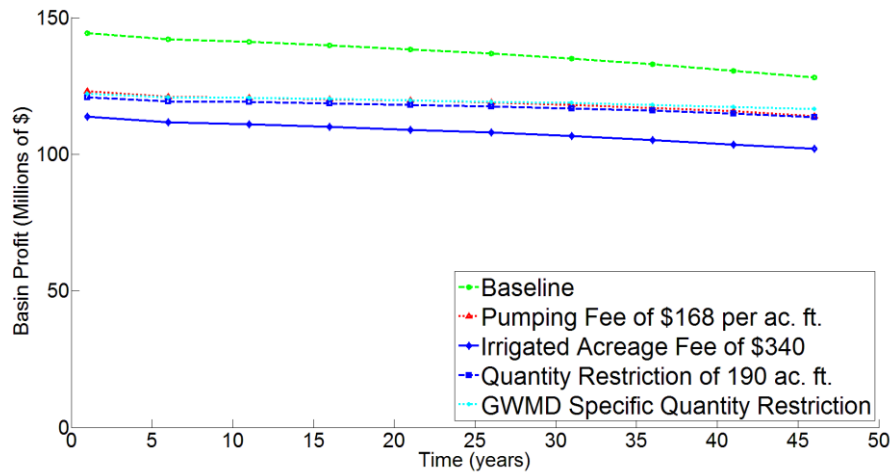
Figure 19: Basin-wide profit under alternative groundwater management policy scenarios.
