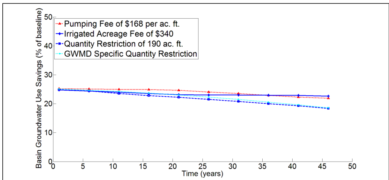
Figure 17: Identifying and comparing water conservation across time under management policies that achieve a 25% reduction in initial pumping levels.
