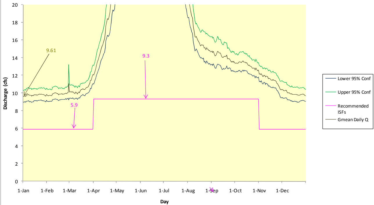
Fig. 2. Geometric Mean Daily Discharge Lower Troublesome Cr abv LT (proportioned on Troublesome Cr nr Pearmont - adj for Irr cons) & ISFs
