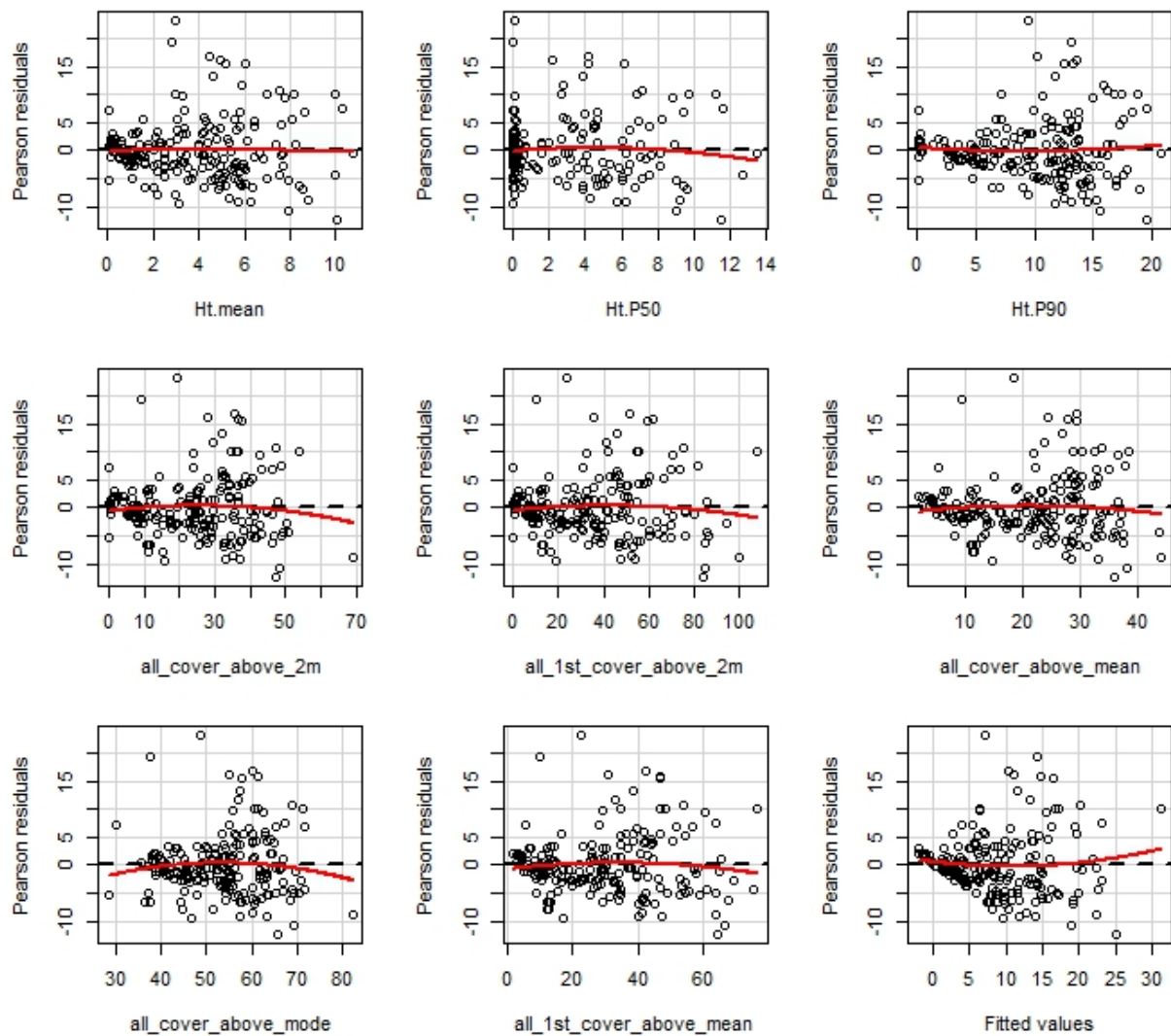
Figure 12: The residuals from the linear model
