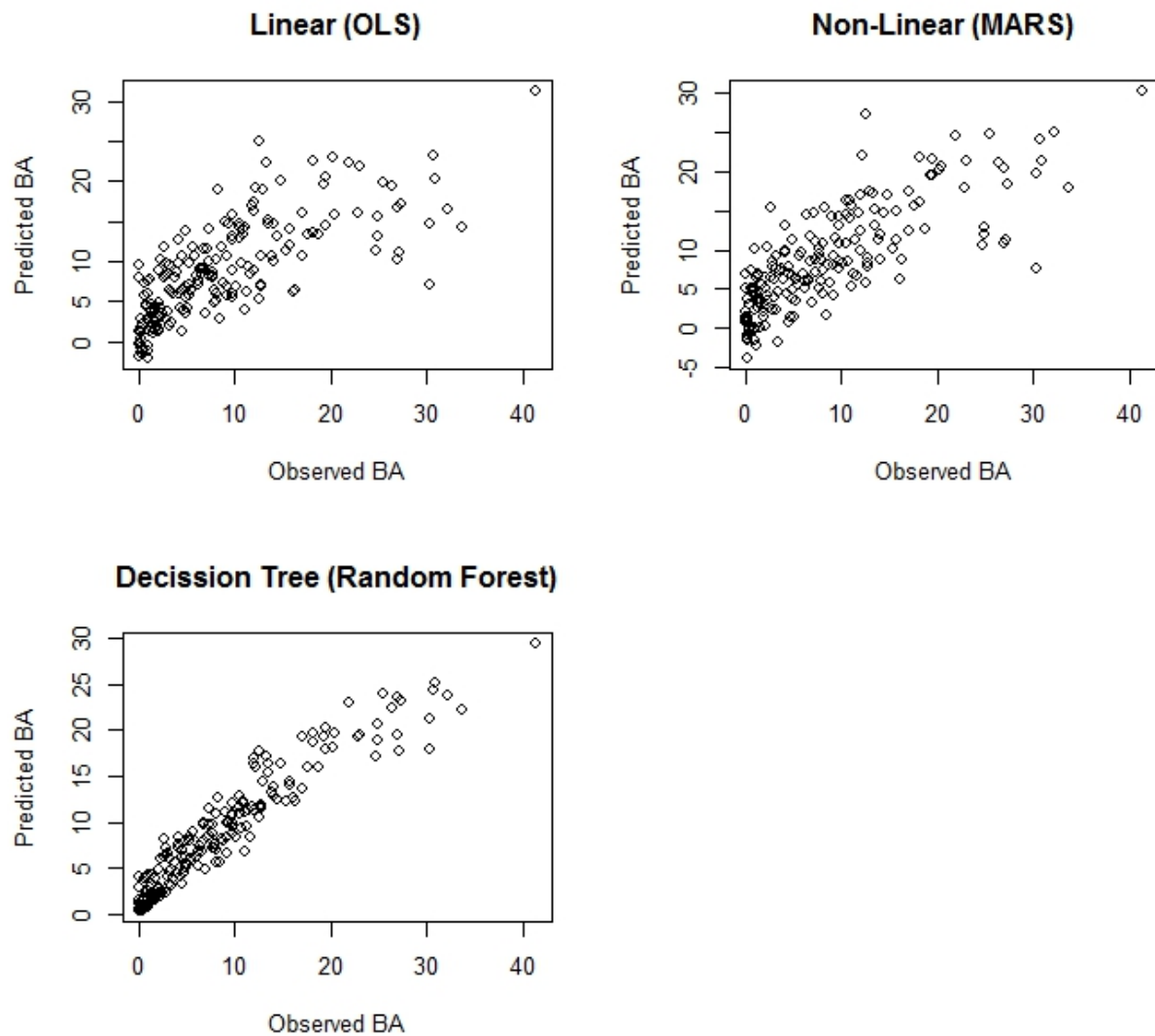
Figure 11: Predicted and Observed values used three different regression models
