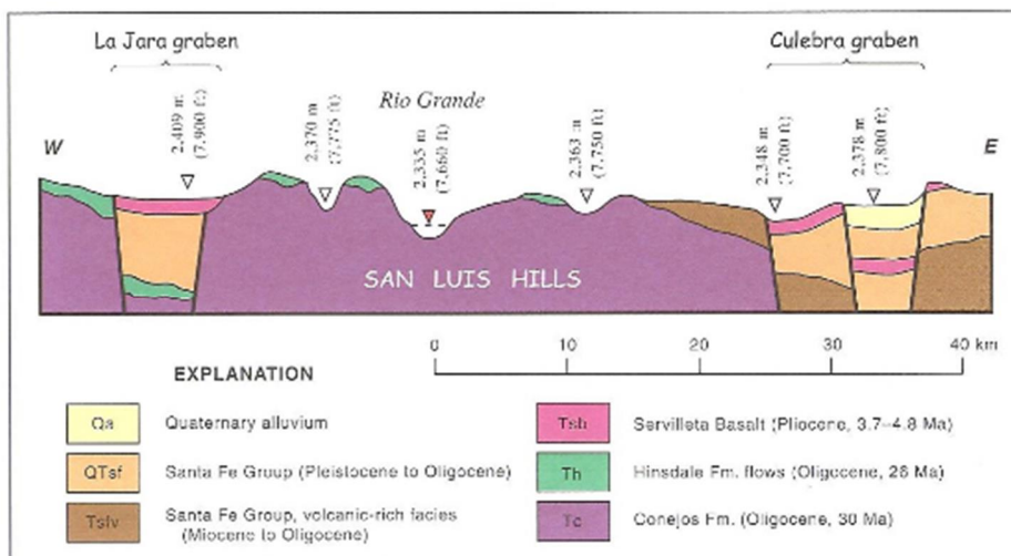
Figure 9. Schematic cross section showing probable Lake Alamosa outlets (topographic lows) adjacent to and within the San Luis Hills along an east-west traverse (location shown in Fig. 2). Eventual outlet through the Fairly Hills sill (dashed line, elevation 2335 m; 7660 ft) shown by red triangle.
