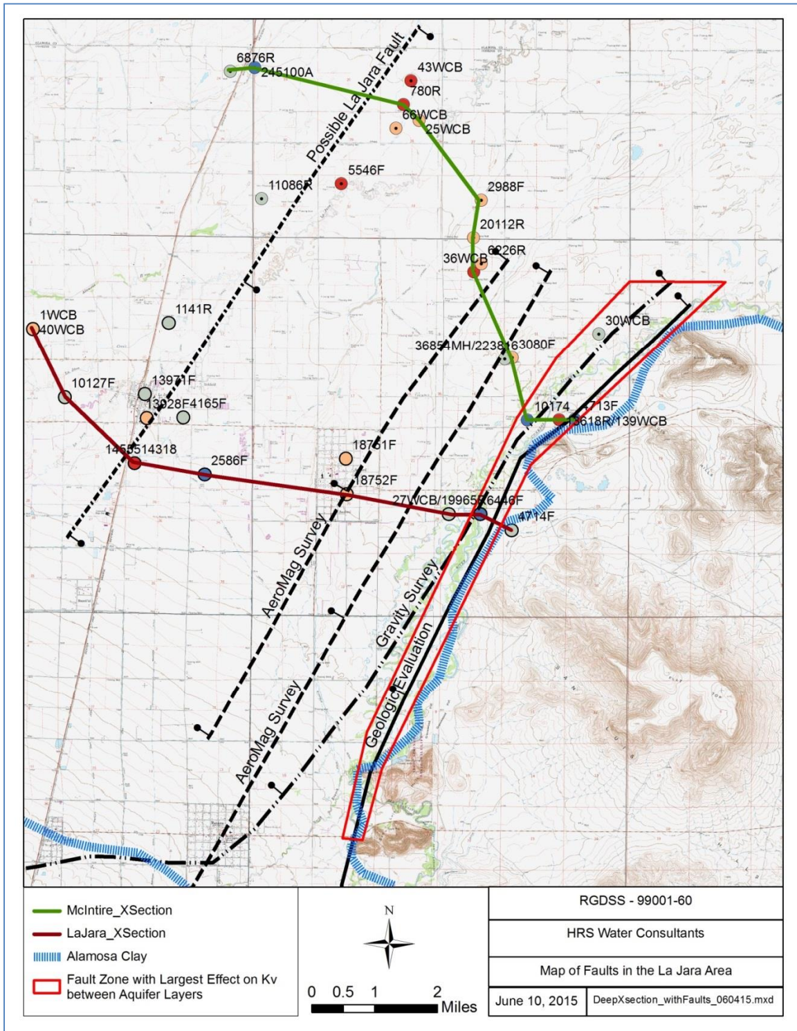
Figure 15. Map of Faults and Cross-Sections
