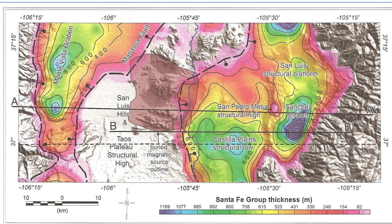
Figure 14. Summary of selected new geologic conclusions determined from geophysical data analysis. Colors and contours indicate estimated thickness of Santa Fe Group sediments from gravity inversion (contour interval 200 m). Locations of newly inferred basin- and graben-bounding normal faults shown by dashed lines with ball on downthrown side. Location of profile model A–A' (Fig. 13) shown, as well as magnetotelluric profile B–B' (Fig. 12).
