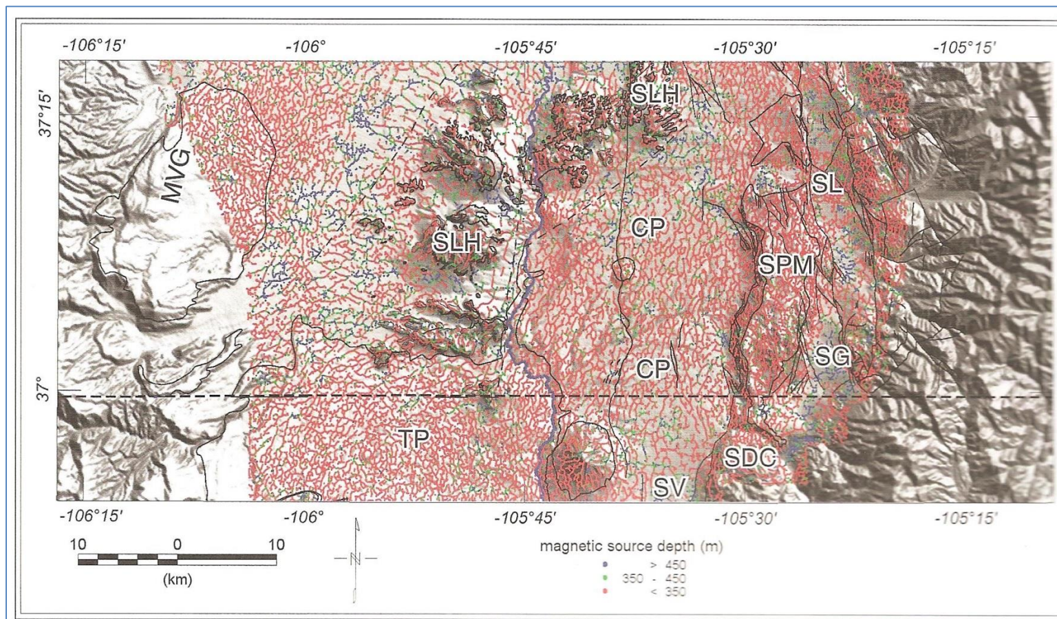
Figure 10: Estimates of depth to magnetic sources, as interpreted by Drenth et al, GSA Special Paper 494, 2013. This figure appeared as Figure 10 in Drenth et al, GSA Special Paper 494, 2013.
