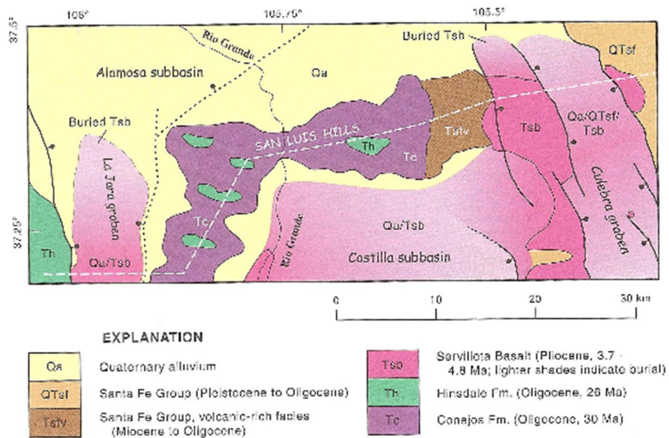
Figure 2. Schematic geologic map of the San Luis Hills showing Pliocene Servilleta Basalt (unit Tsb) that flowed northward around east and west margins of the hills. Slashes indicate stacked units (e.g., Qa/Tsb indicates Qa over Tsb). White dashed line shows topographic divide of Figure 9.
