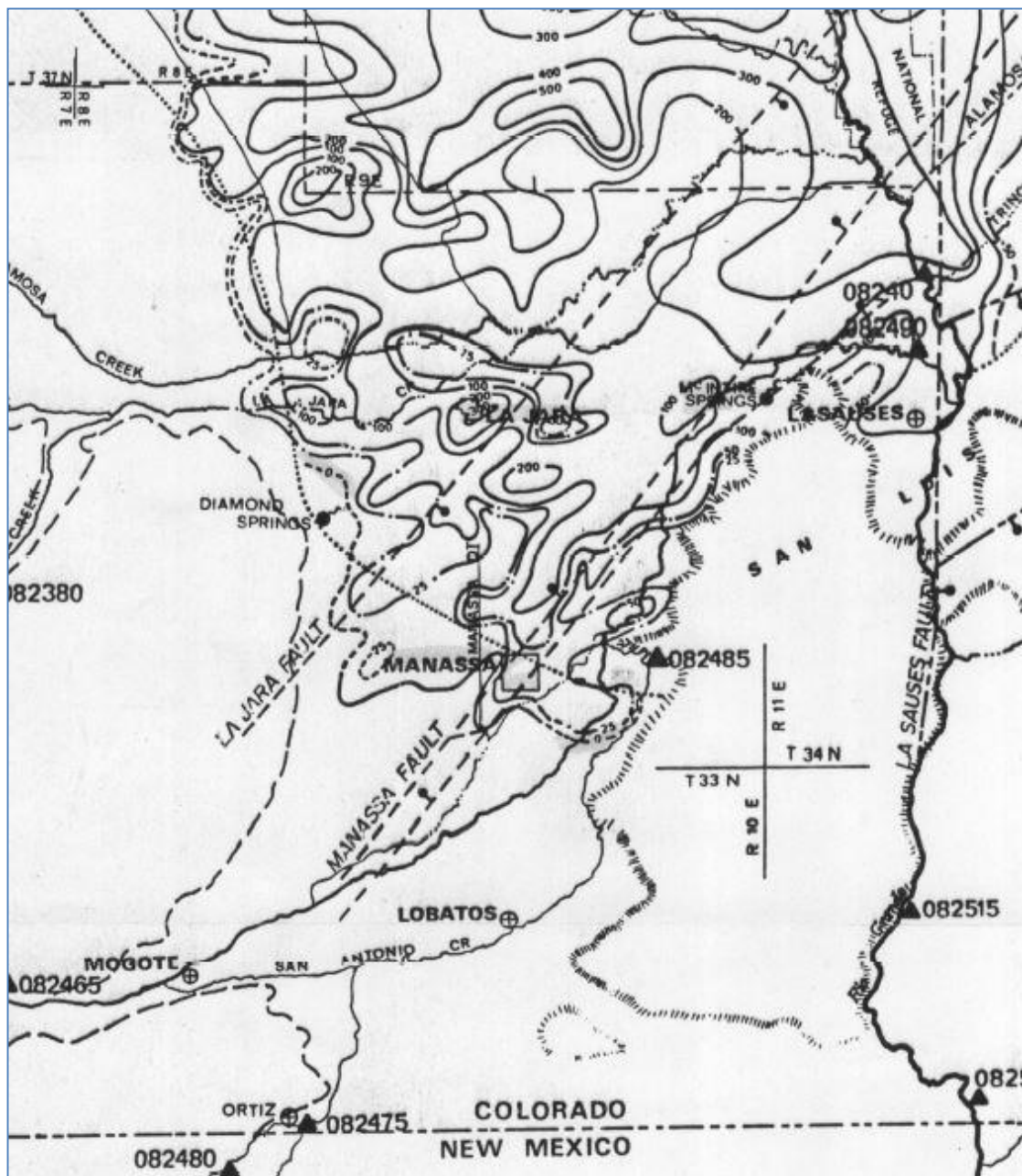
Figure 8: Excerpt from Moravec, G., and Schroeder, D., 1978, Isopach Map of the Blue Clay Series, Plate 5-1, Colorado Division of Water Resources.
