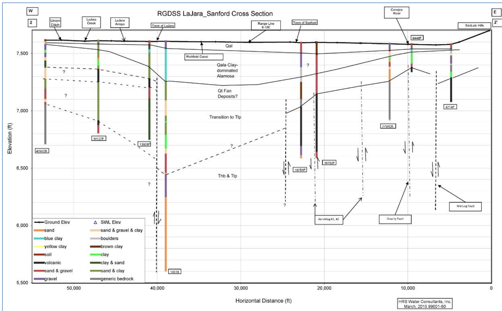
Figure 14. LaJara-Sanford Cross-Section
