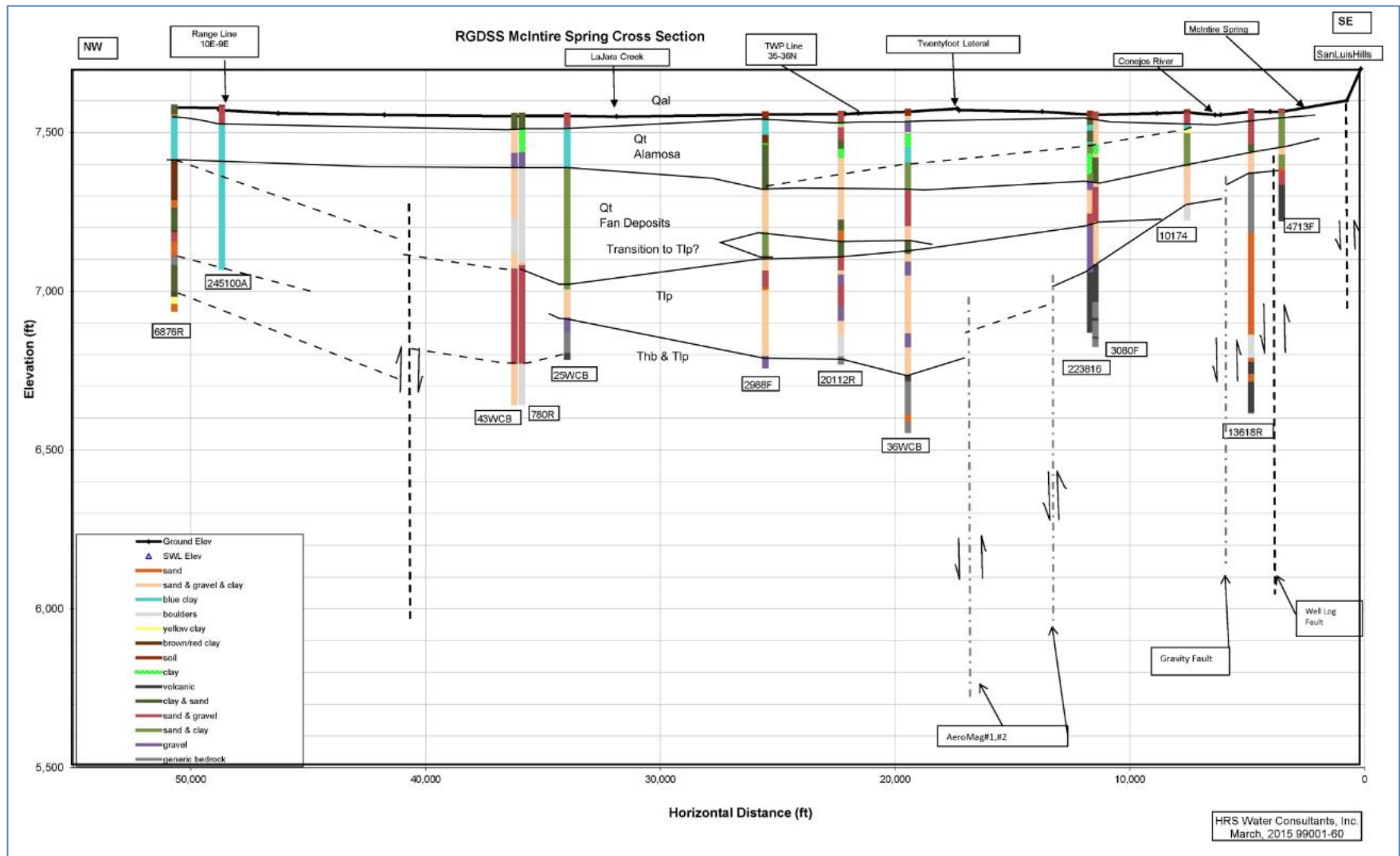
Figure 13. McIntire Spring Cross-Section
