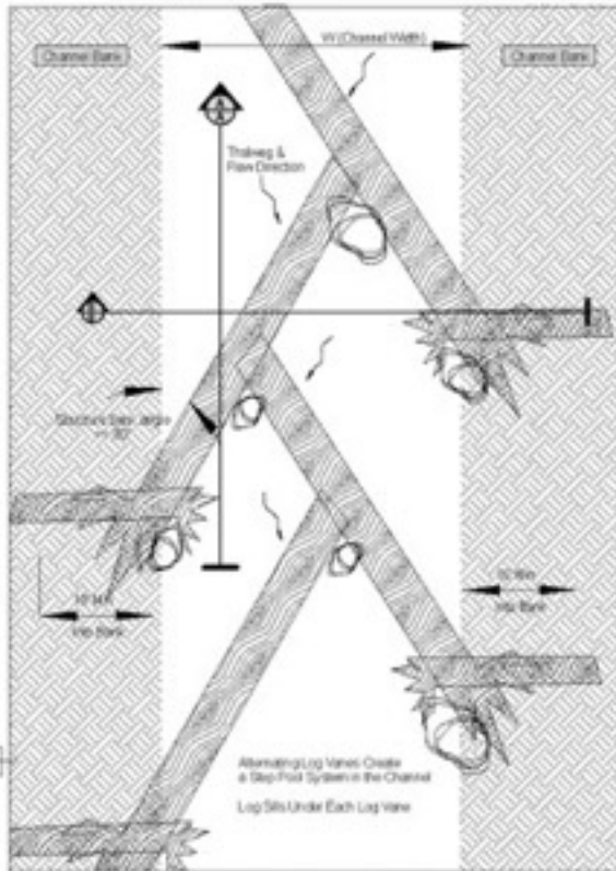
Detail Drawing #6 - Log Rock & Roll Structure Plan View Not To Scale
