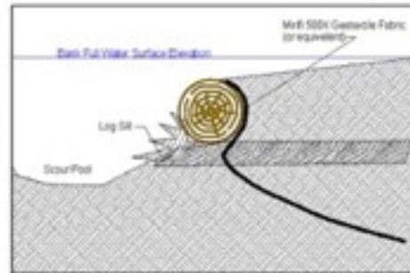
Long A-A Log Vane Profile Not To Scale
