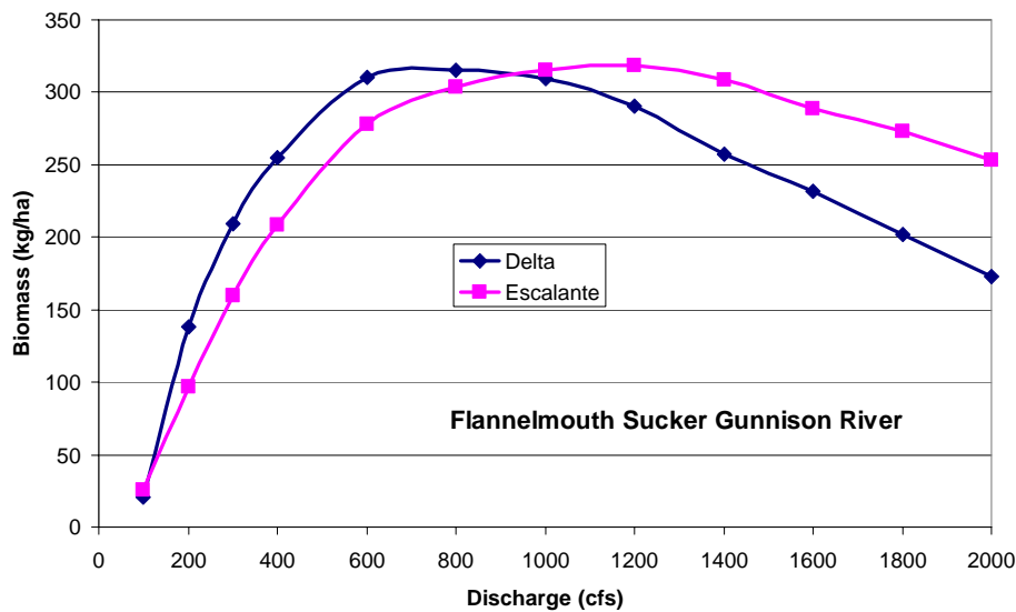
Figure 5. Modeled flannemouth sucker biomass (kg/ha) as a function of discharge, Delta and Escalante, Gunnison River.
