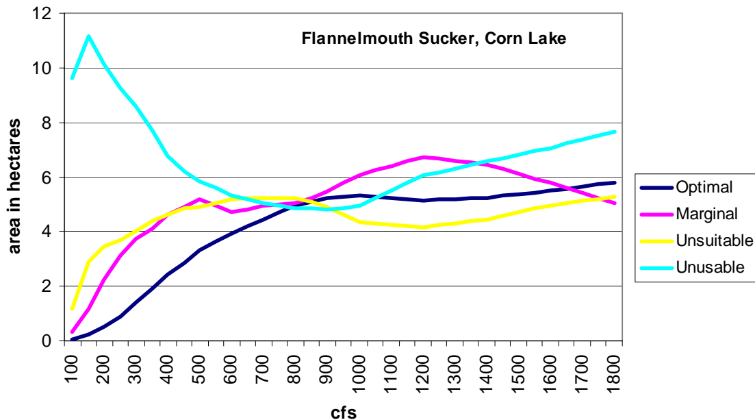
Figure 17. Flannemouth sucker habitat availability at Corn Lake, Colorado River.
