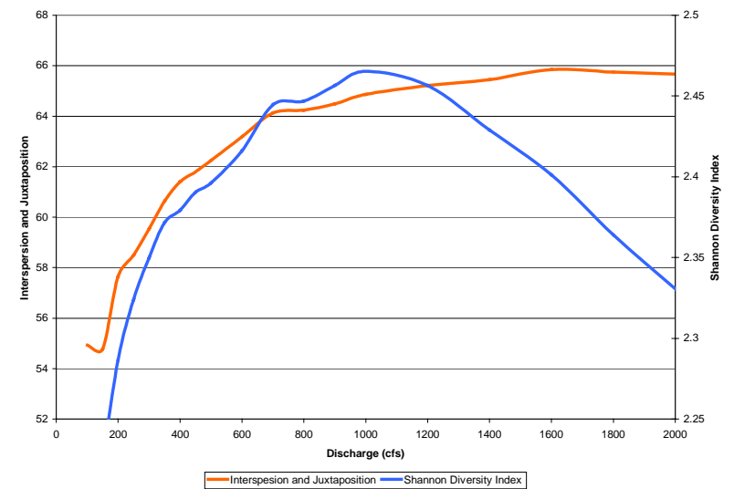
Figures A11 a, b, c, d. Meso-habitat and Shannon Diversity and Interspersed for modeled flows at Corn Lake (above) and Clifton, Colorado River.
