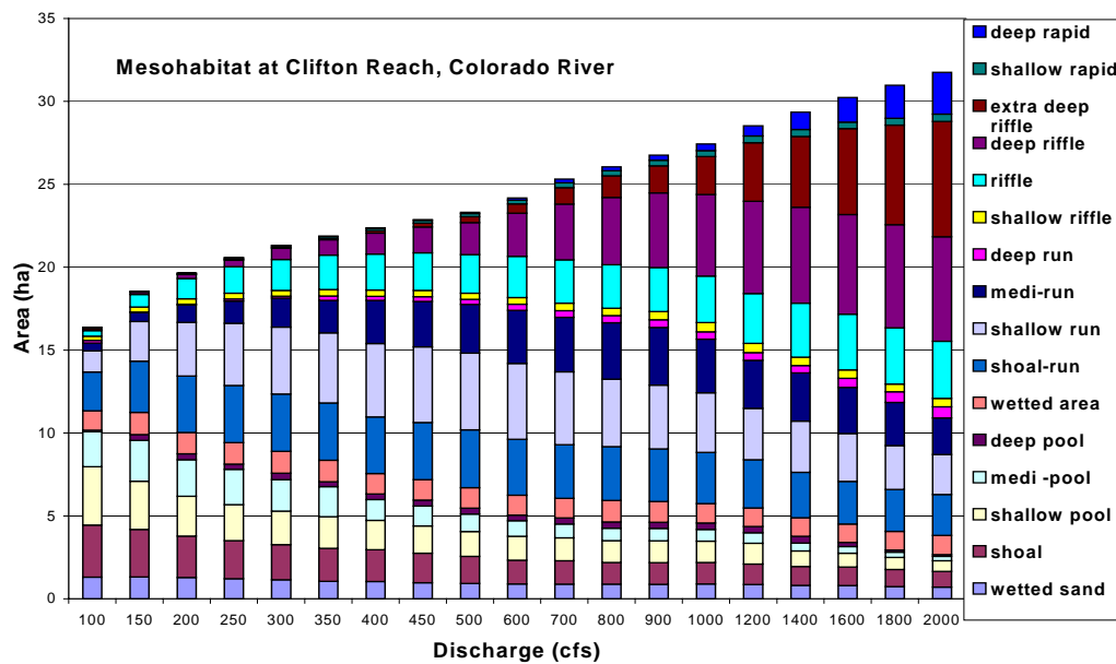
Figures A11 a, b, c, d. Meso-habitat and Shannon Diversity and Interspersed for modeled flows at Corn Lake (above) and Clifton, Colorado River.
