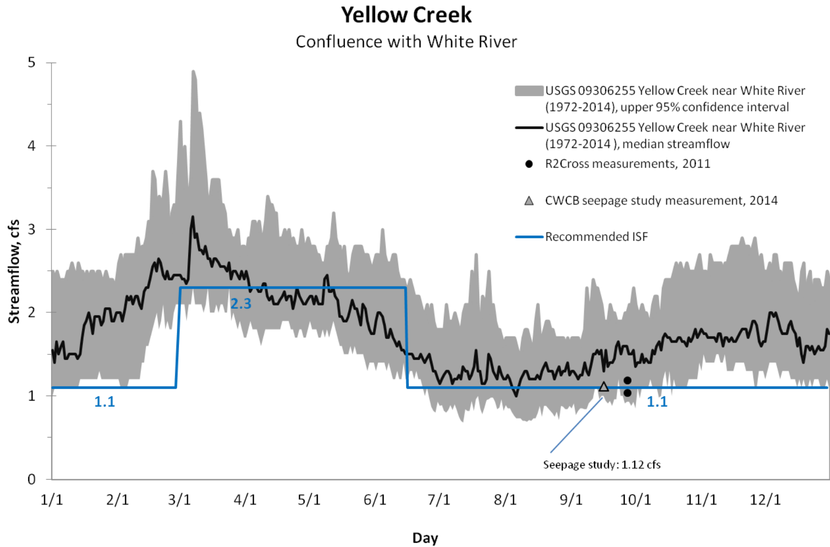
Figure 1. Complete hydrograph showing streamflow data and the proposed ISF rate on lower Yellow Creek.
