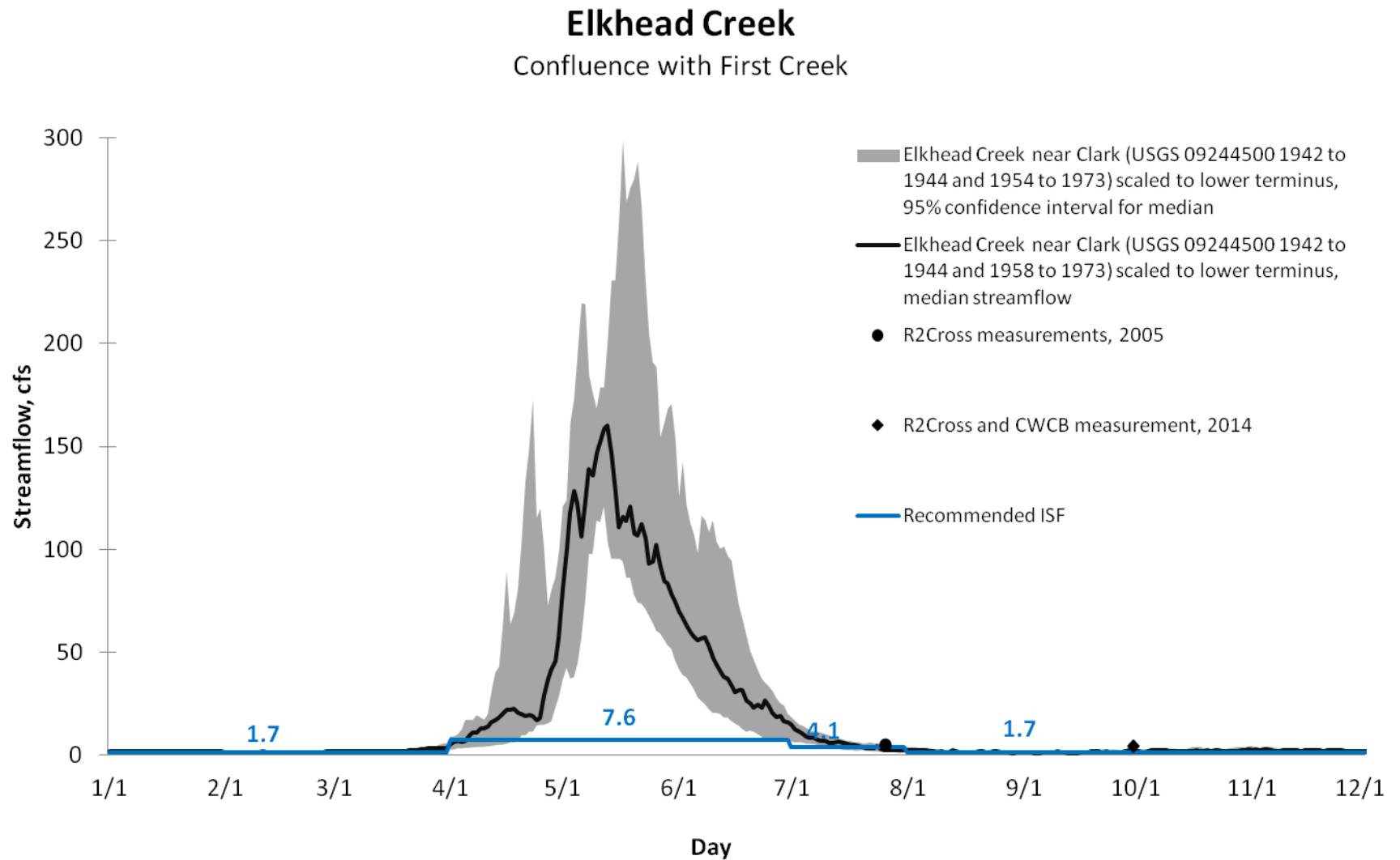
Figure 1. Complete hydrograph showing streamflow data and the proposed ISF rate on Elkhead Creek.
