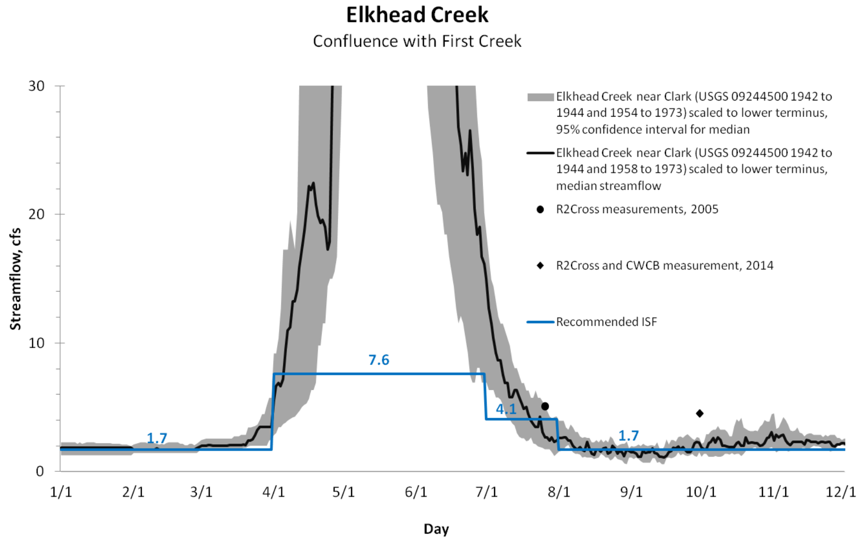
Figure 2. Detailed hydrograph showing streamflow data and the proposed ISF rate on Elkhead Creek.
