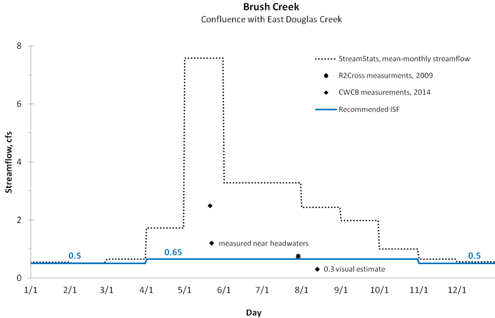
Figure 1. Complete hydrograph showing streamflow data and the proposed ISF rate on Brush Creek.
