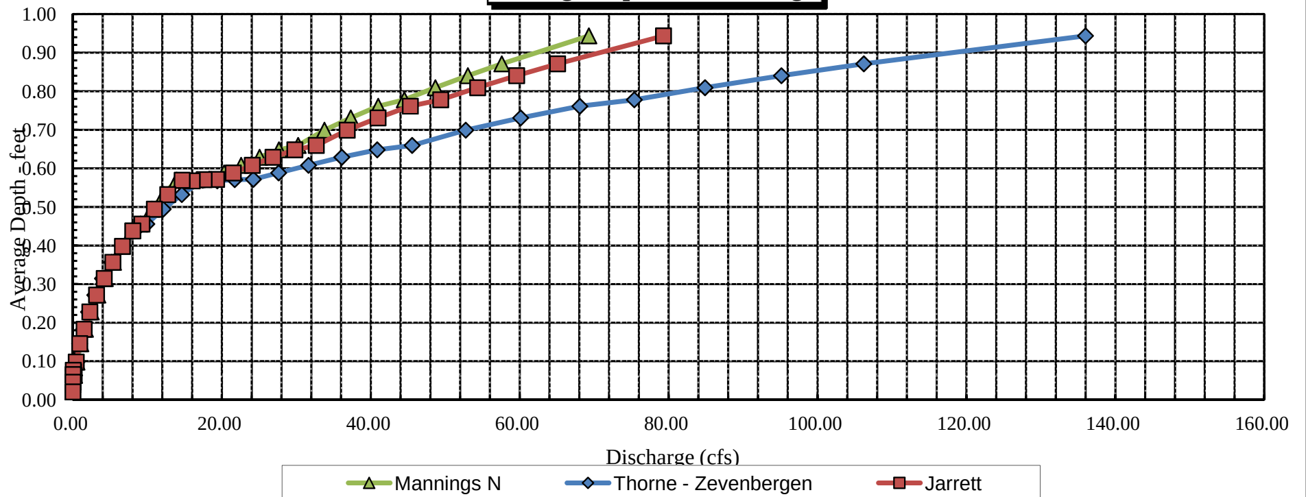
Schaefer Creek Average Depth vs. Discharge
