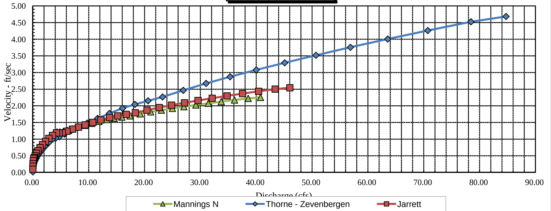
Schaefer Creek Velocity vs. Discharge
