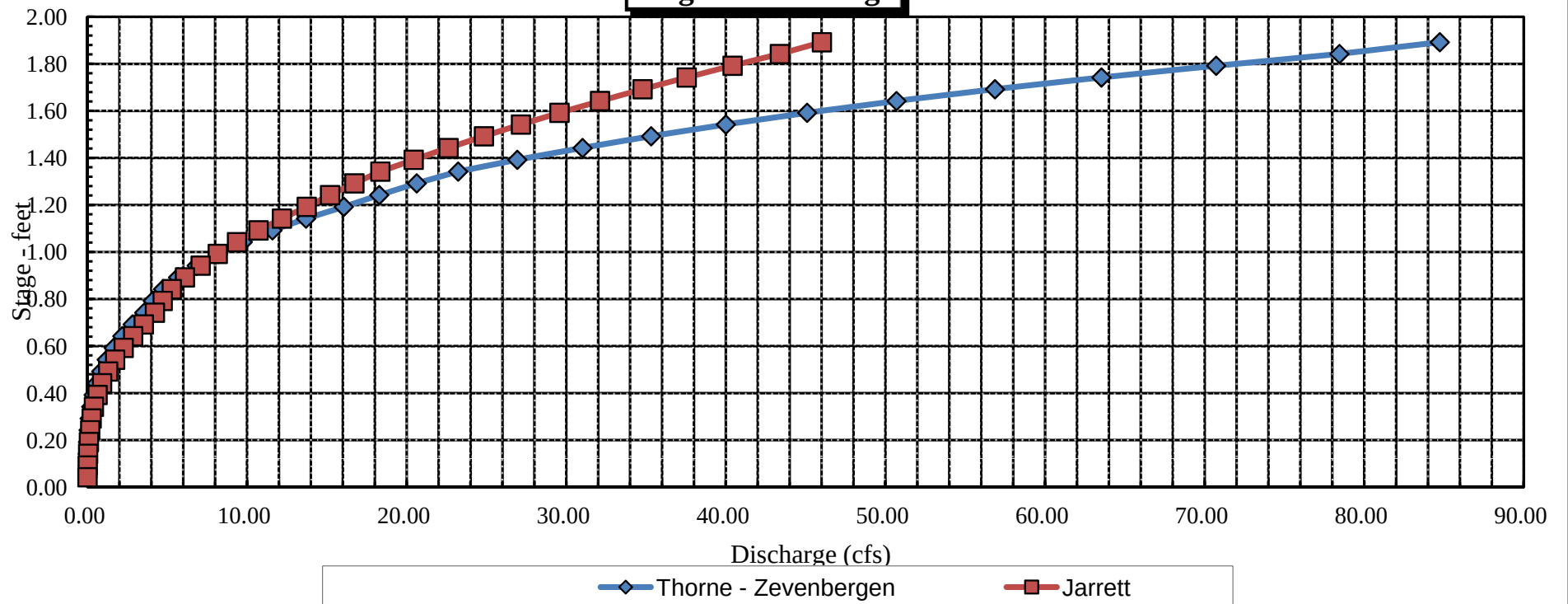
Schaefer Creek Stage vs. Discharge
