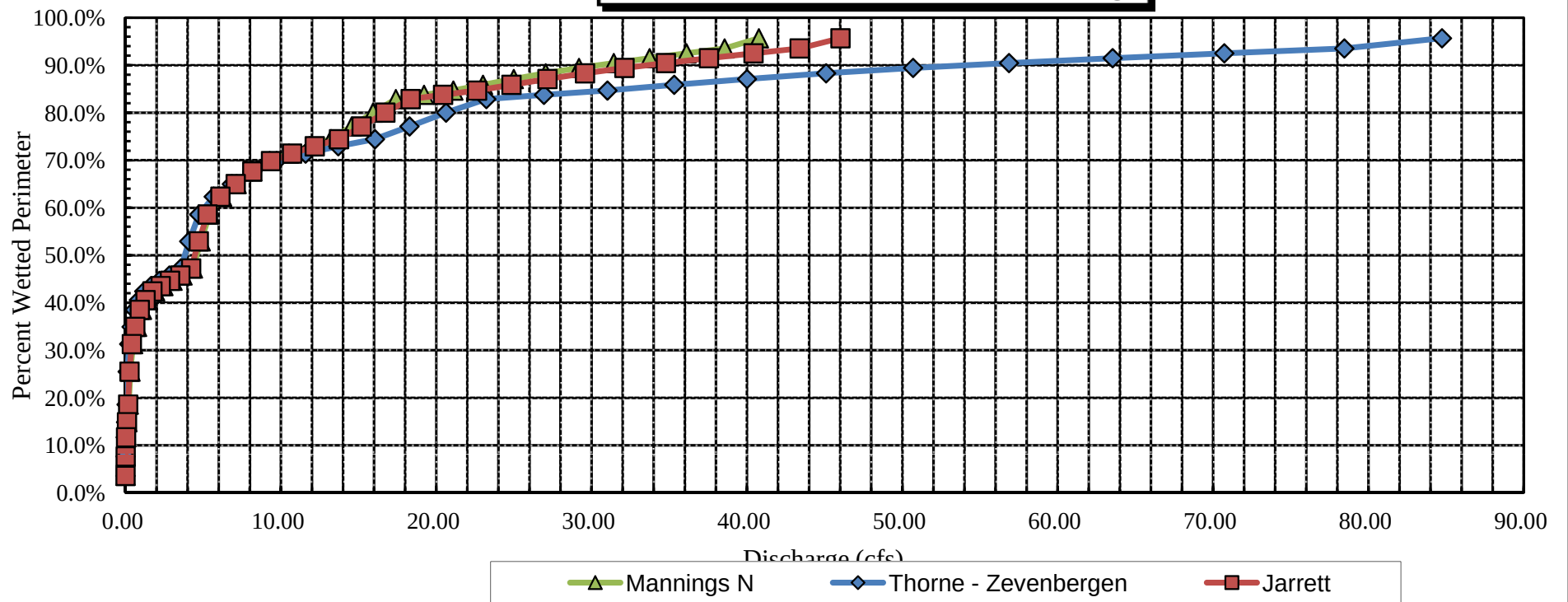
Schaefer Creek Percent Wetted Perimeter vs. Discharge
