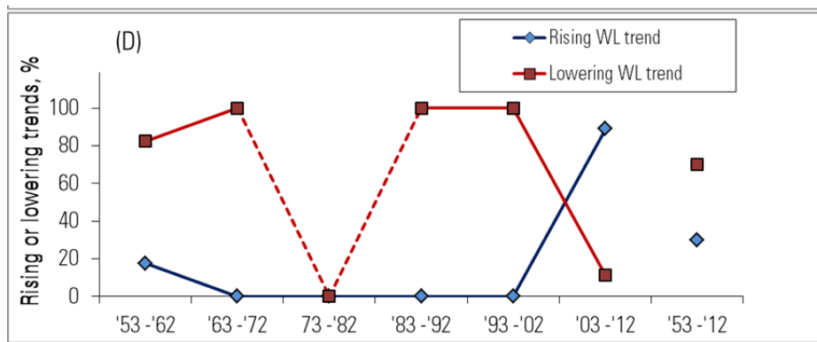
Percentage of Wells by Decade Having Rising or Lowering Water Level Trends. (insufficient data for the decade of '73-'82)
