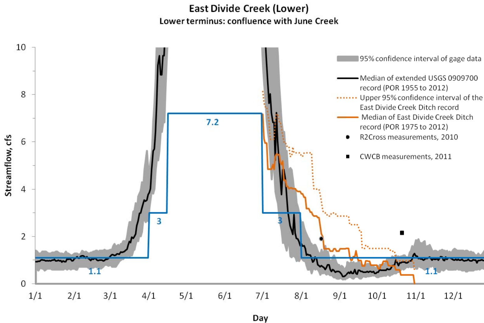
Figure 1. Hydrograph showing streamflow data, diversion data, and the proposed ISF flow on the lower segment of East Divide Creek.
