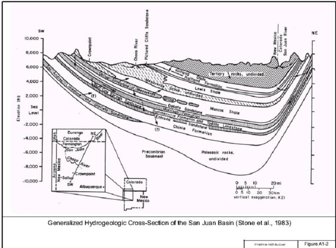
Figure 5. Cross sectional geology. The Animas flows across the anticline (Fruitland Outcrop) shown at the right of the figure.
