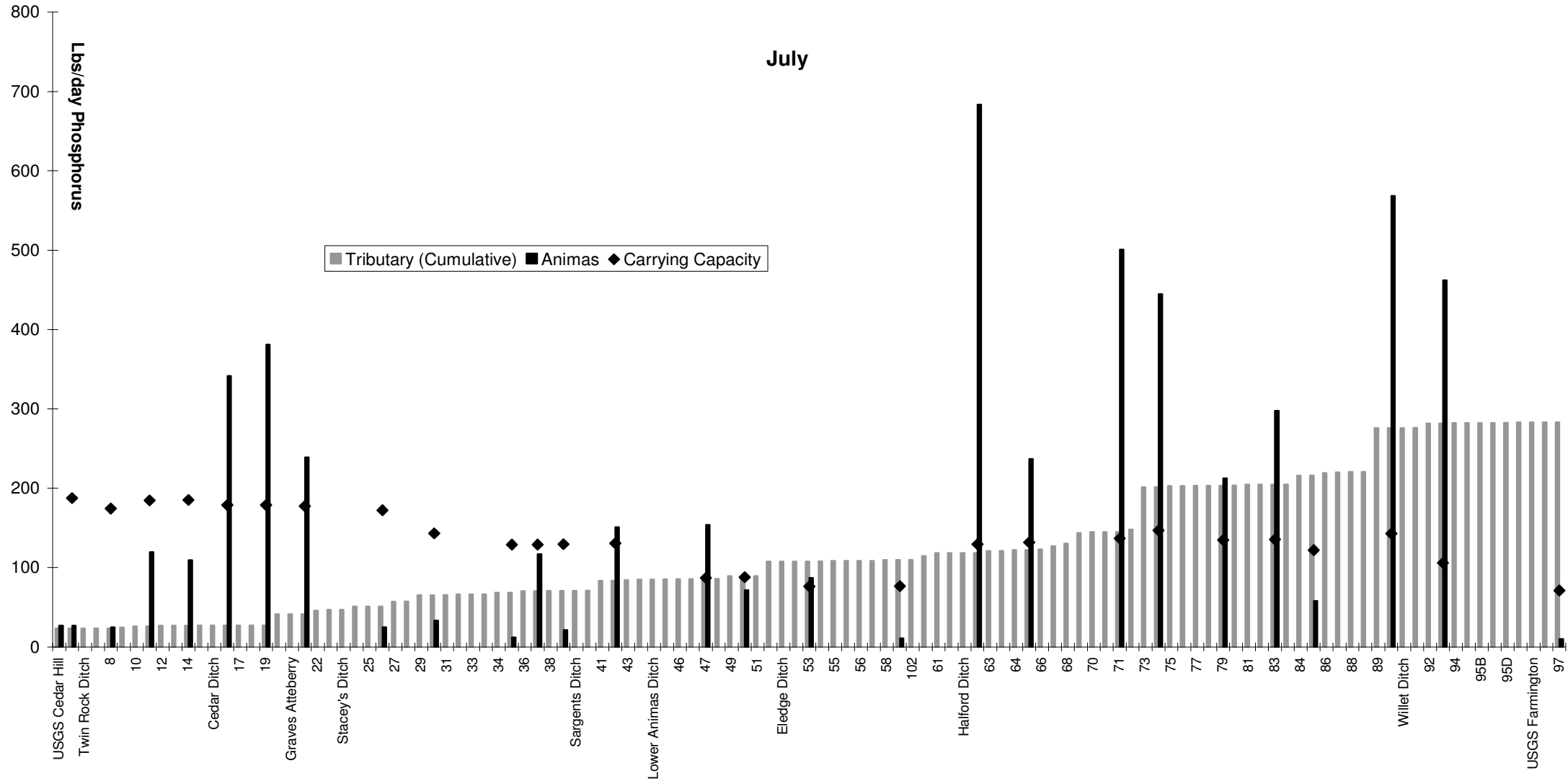
Figure 14. July 2006 total phosphorus loading. Grey bars are cumulative loading from inflows, black bars are measured loading into the Animas River and black diamonds are calculated carrying capacity of the Animas River (all units are lbs/d, see Figure 1 for Animas River flow estimates, see Table 12 & Table 13 for data.
