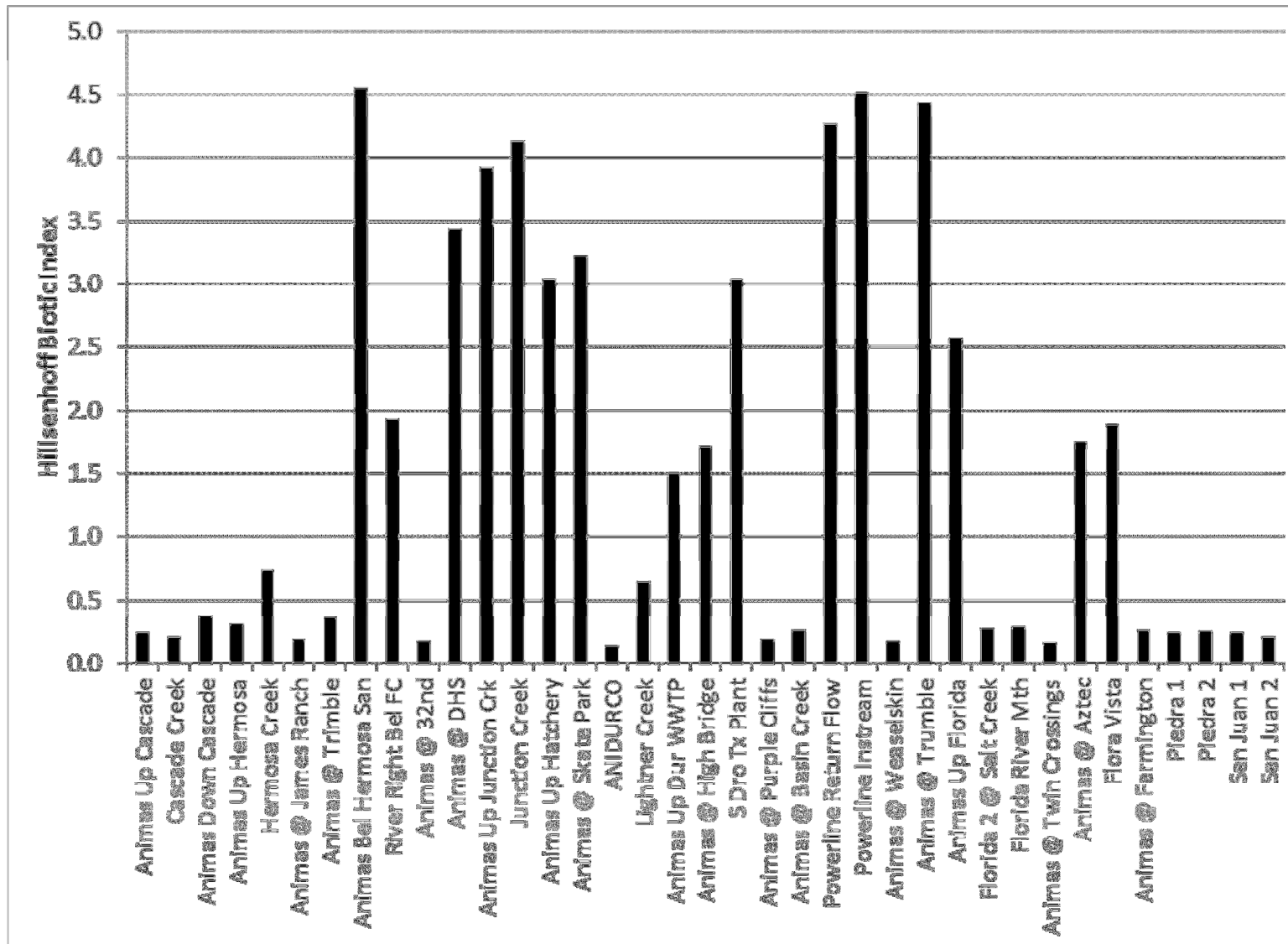
Figure 22. Hilsenhoff Biotic Index for benthic macroinvertebrates. The HBI value represents the tolerance of benthic macroinvertebrates to pollution. High values indicate high tolerance to pollution; therefore, low values are the desirable condition. It is recommended that the Stakeholders establish a goal of less than 2 throughout the river.
