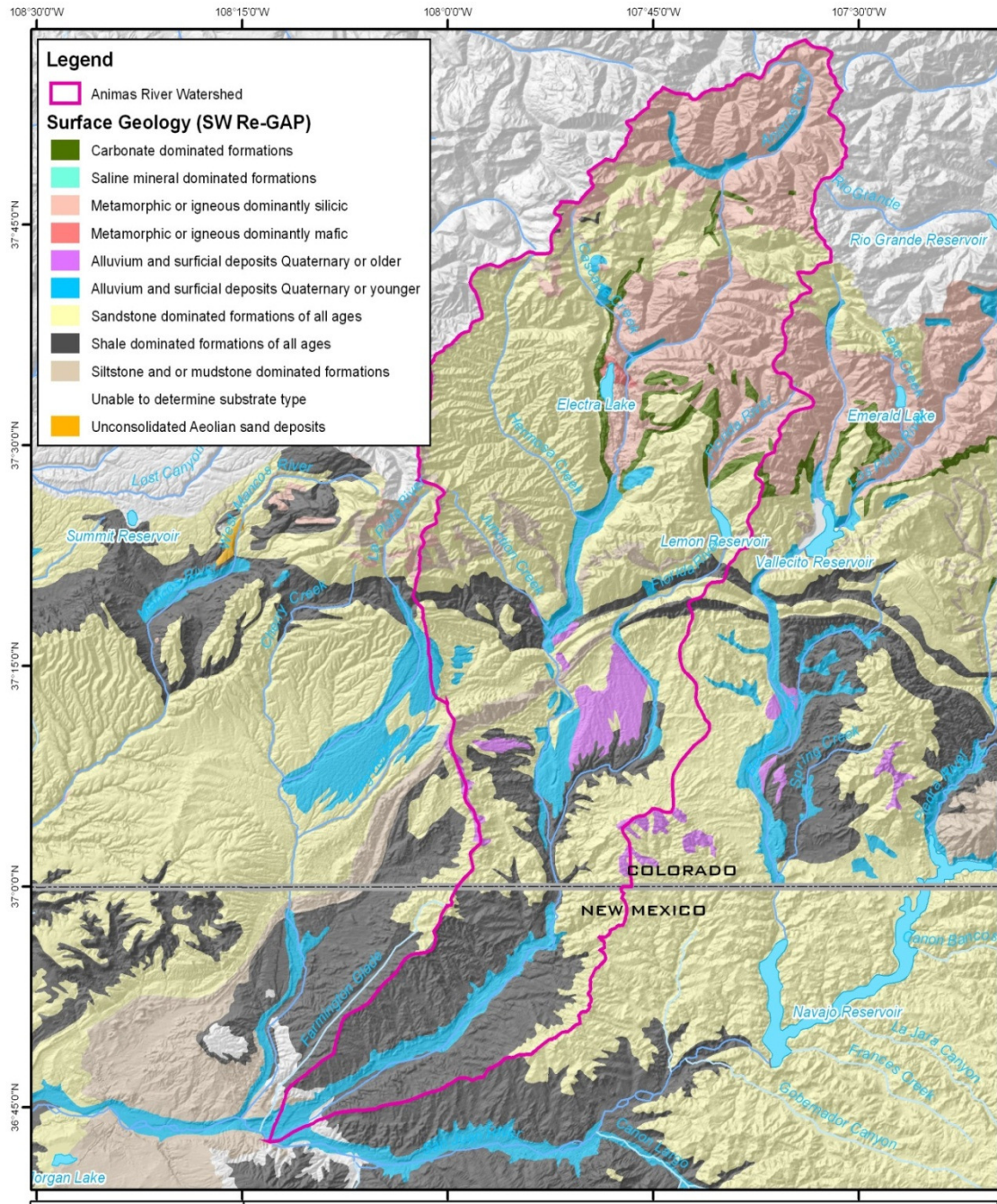
Figure 4. Surface geology in the Animas River Watershed.
