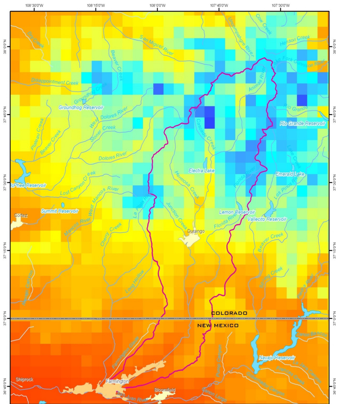
Figure 7. 100 year average of annual precipitation in the Animas River Watershed.
