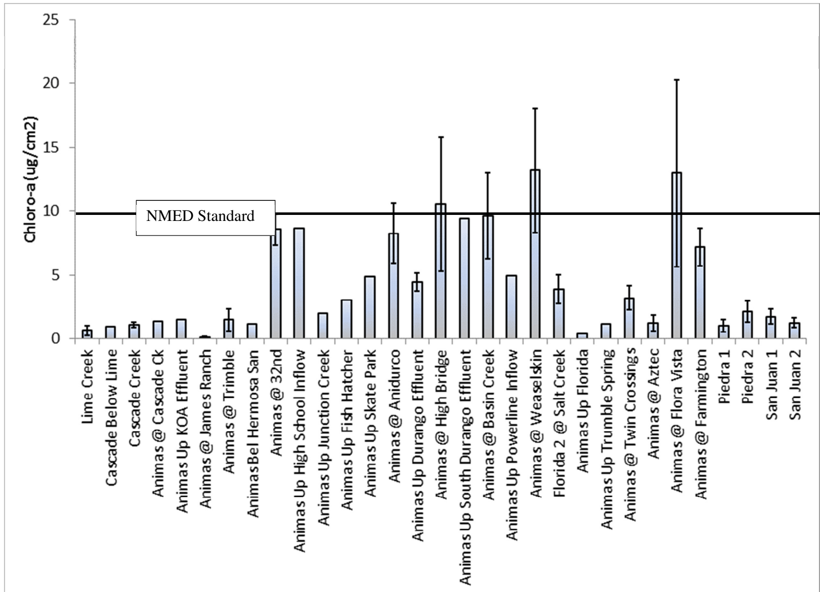
Figure 21. Average periphyton biomass ( \pm standard error) measured as chlorophyll-a. The NMED standard is 10ug/cm2.
