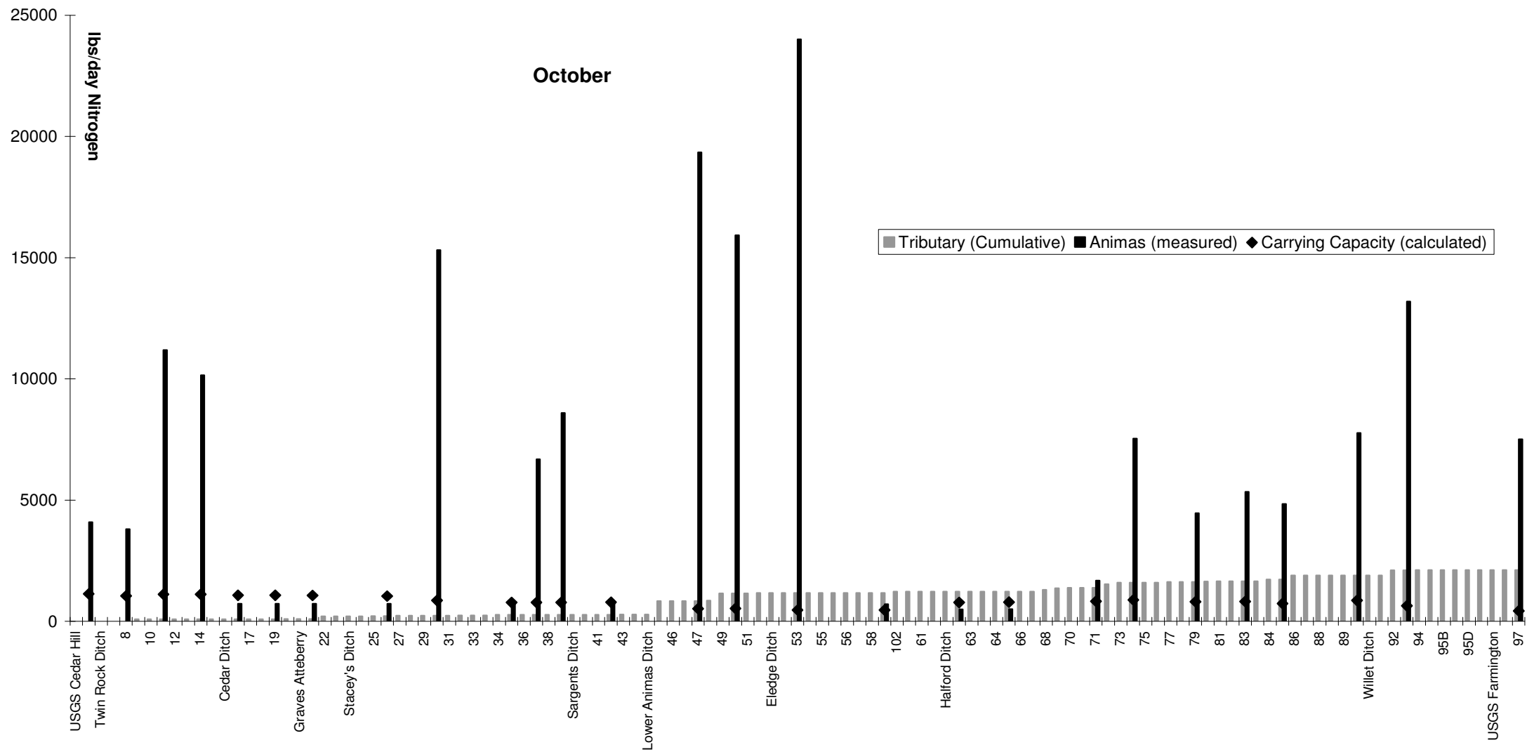
Figure 15. October 2006 total nitrogen loading. Grey bars are cumulative loading from inflows, black bars are measured loading into the Animas River and black diamonds are calculated carrying capacity of the Animas River (all units are lbs/d, see Figure 2 for Animas River flow estimates, see Table 12 & Table 13 for data).
