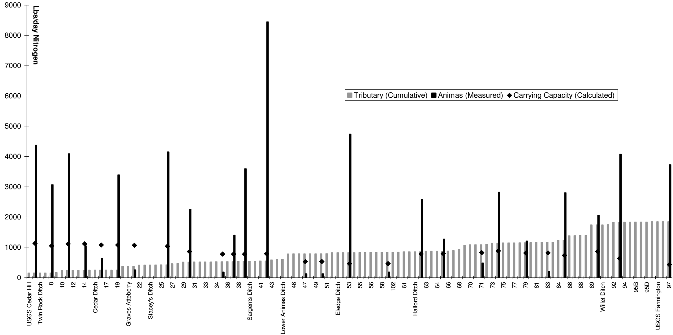
Figure 13. July 2006 total nitrogen loading. Grey bars are cumulative loading from inflows, black bars are measured loading into the Animas River and black diamonds are calculated carrying capacity of the Animas River (all units are lbs/d, see Figure 1 for Animas River flow estimates, see Table 12 & Table 13 for data).
