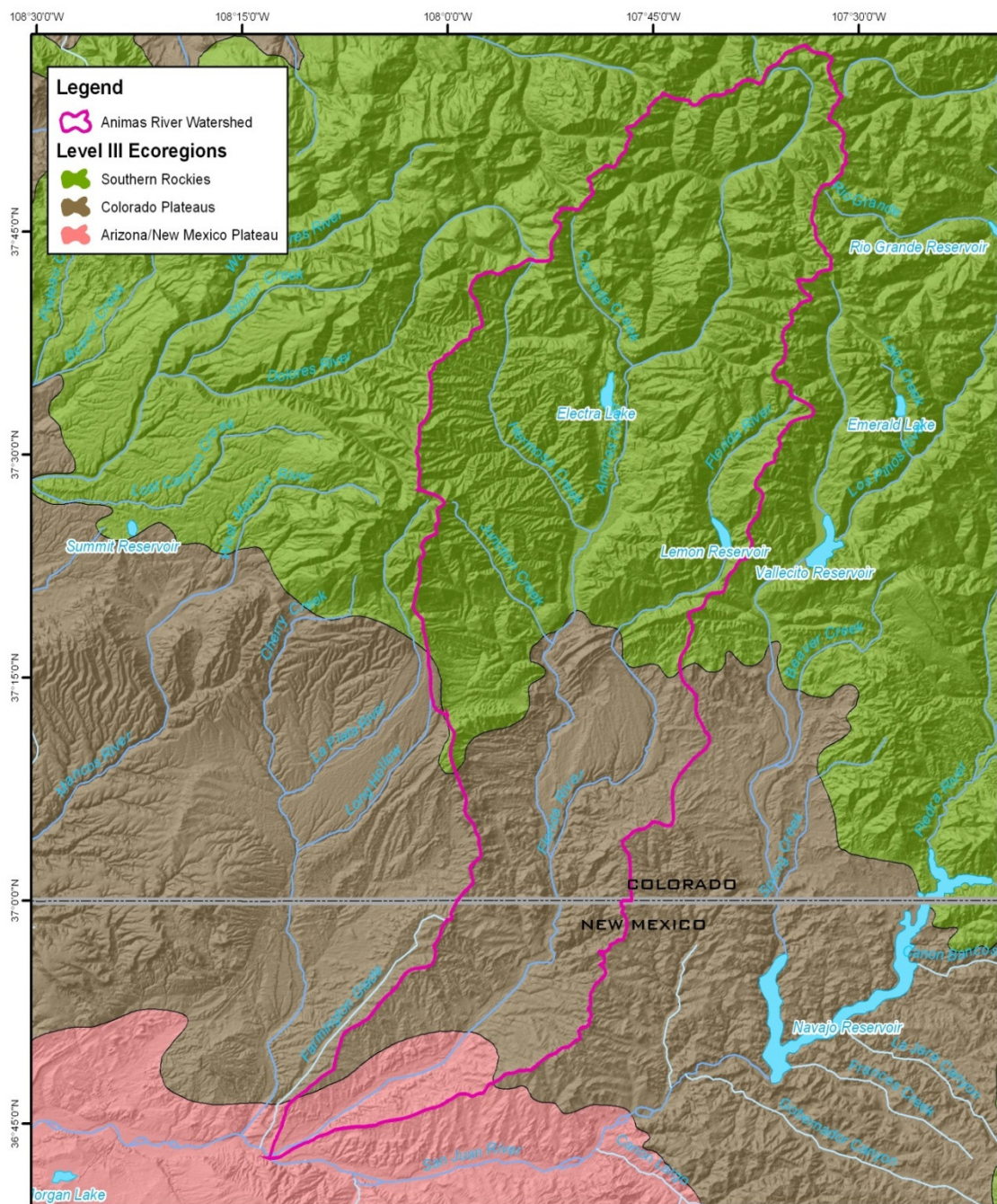
Figure 6. Ecoregions of Animas River Watershed, Level III.
