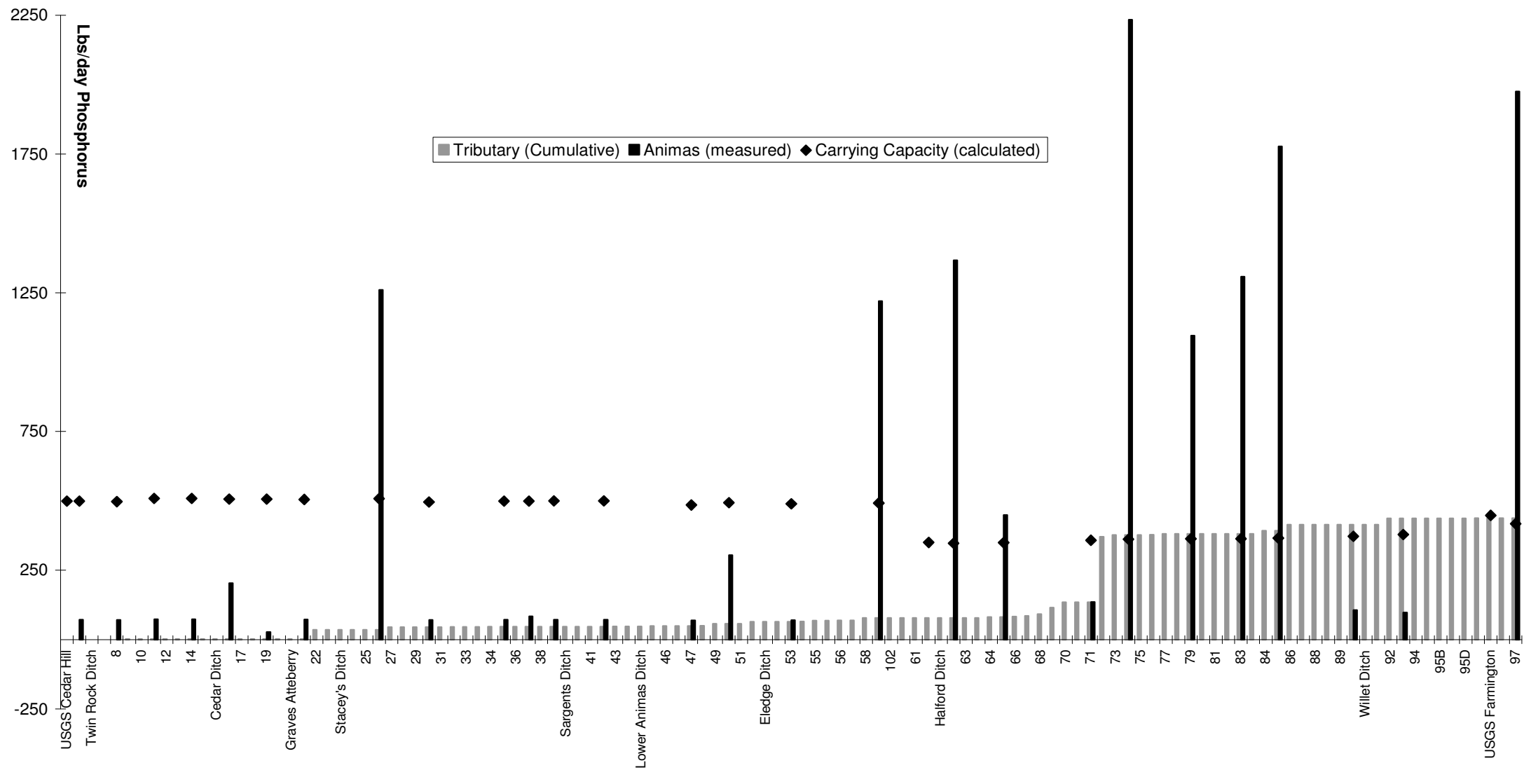
Figure 16. October 2006 total phosphorus loading. Grey bars are cumulative loading from inflows, black bars are measured loading into the Animas River and black diamonds are calculated carrying capacity of the Animas River (all units are lbs/d, see Figure 2 for Animas River flow estimates, see Table 12 & Table 13 for data).
