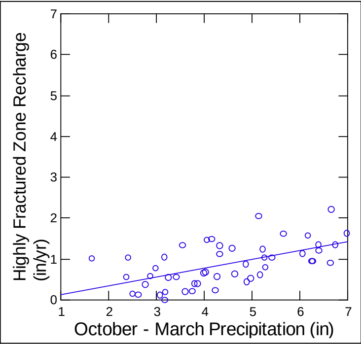
Figure 3-12 Relationship between Winter Precipitation and Highly Fractured Zone Recharge
