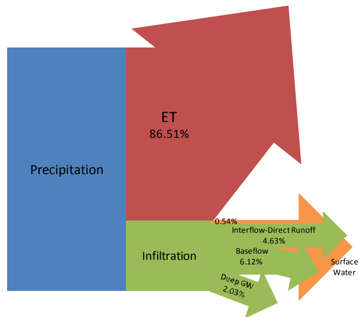
Figure 3-9 Precipitation Partitioning based on Turkey Creek Study
