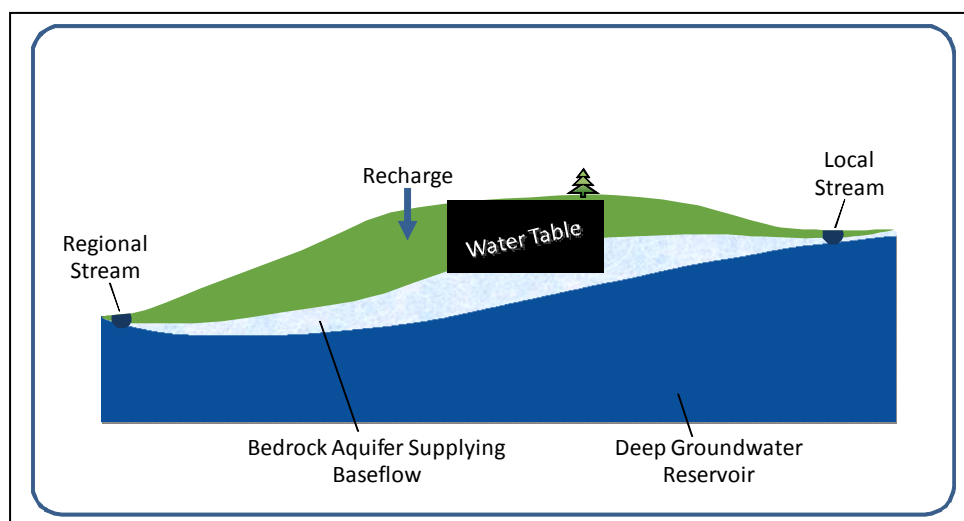
Figure 3-8 Schematic Representation of Baseflow and Deep Groundwater Reservoirs
