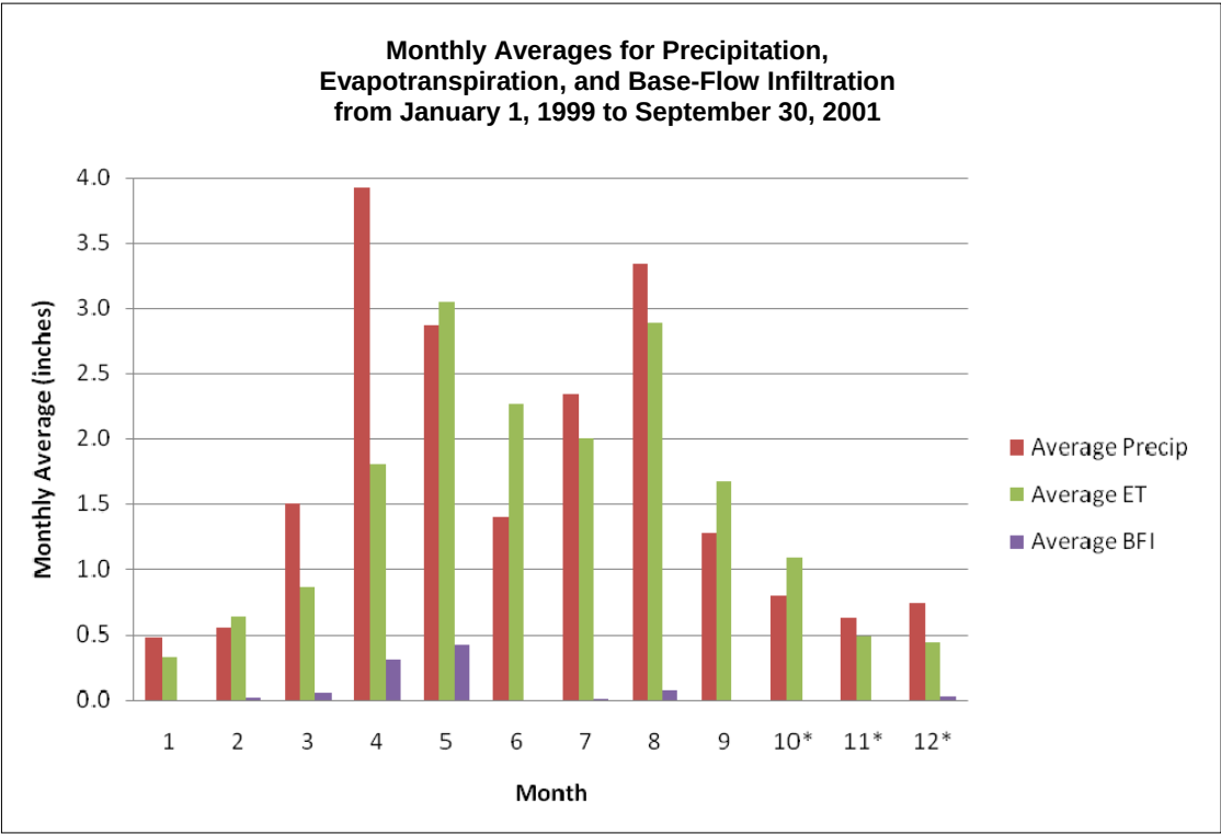
Figure 3-4 Comparison of Turkey Creek Precipitation, Evapotranspiration, and Recharge
