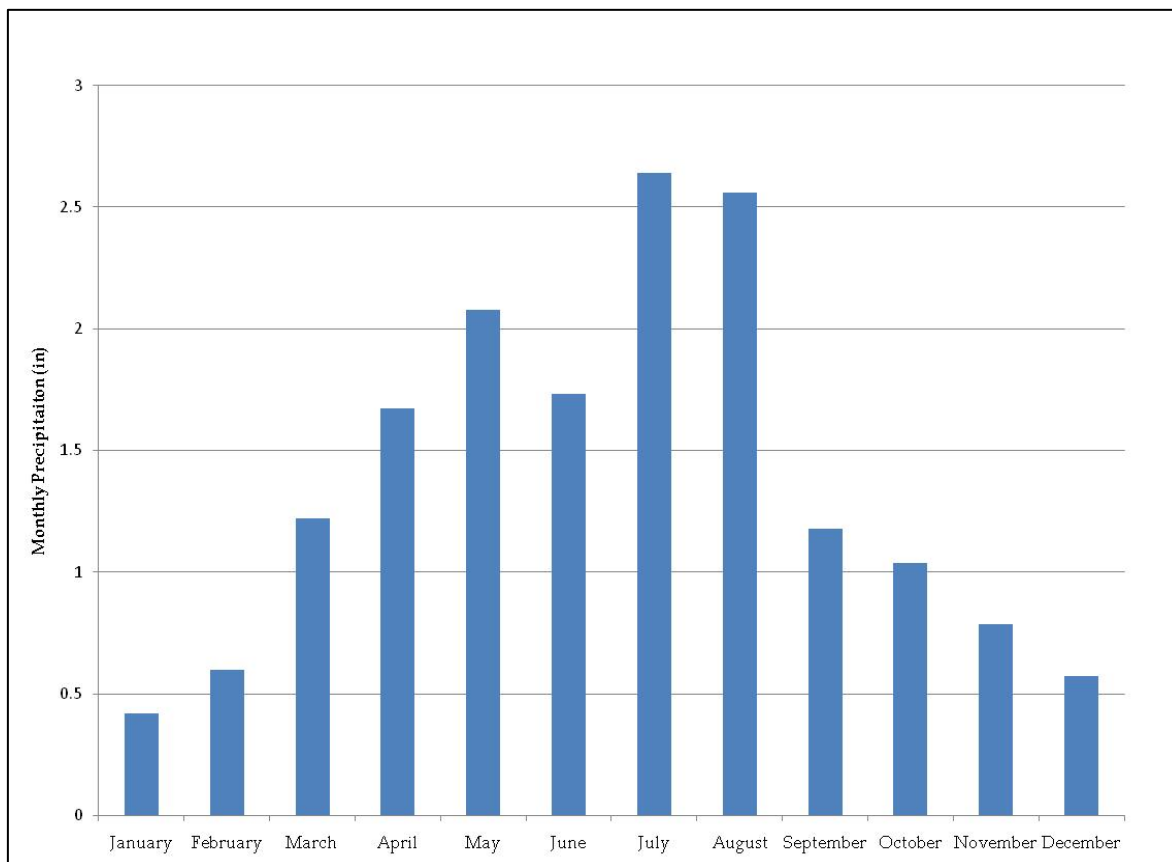
Figure 3-3 Average Monthly Precipitation at Cheesman Dam from 1949 to 1999
