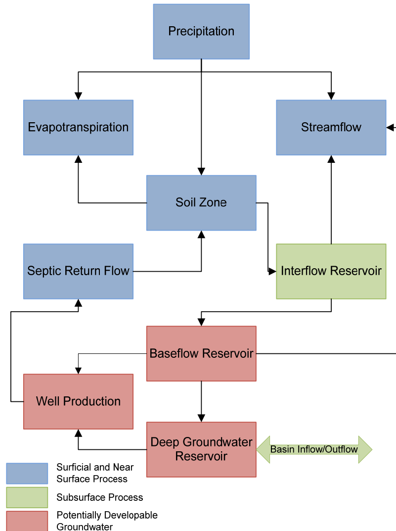
Figure 3-7 Site Water Budget Conceptual Model
