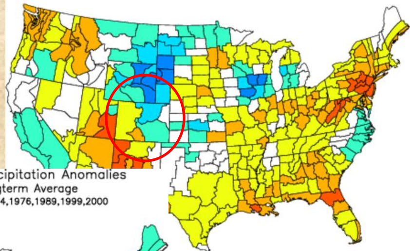
Composite Standardized Precipitation Anomalies Versus 1950–1995 Longterm Average Apr 1950,1955,1956,1967,1971,1974,1976,1989,1999,2000 2008
