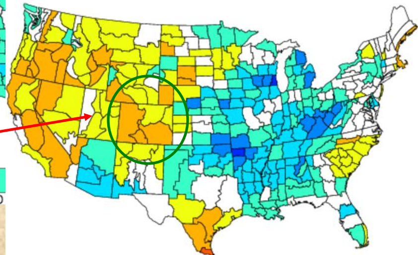
Composite Standardized Precipitation Anomalies Versus 1950–1995 Longterm Average Jun 1950,1955,1956,1967,1971,1974,1976,1989,1999,2000 2008
