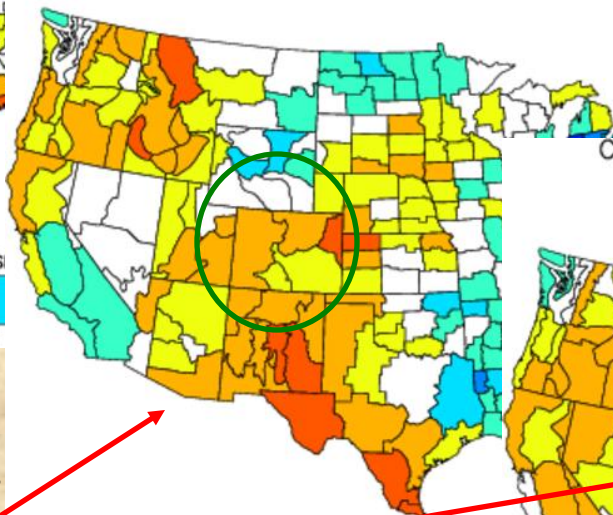
Composite Standardized Precipitation Anomalies Versus 1950–1995 Longterm Average May 1950,1955,1956,1967,1971,1974,1976,1989,1999,2000 2008
