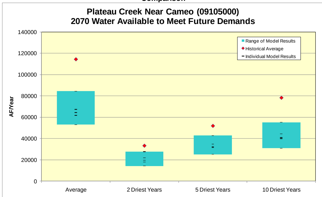
Figure F139 –2070 Plateau near Cameo Water Available to Meet Future Demands Low-flow Comparison
