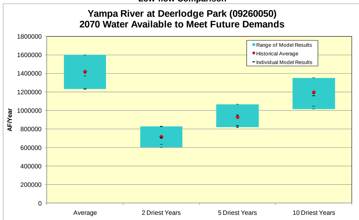
Figure F167 –2070 Yampa River at Deerlodge Park Water Available to Meet Future Demands Low-flow Comparison
