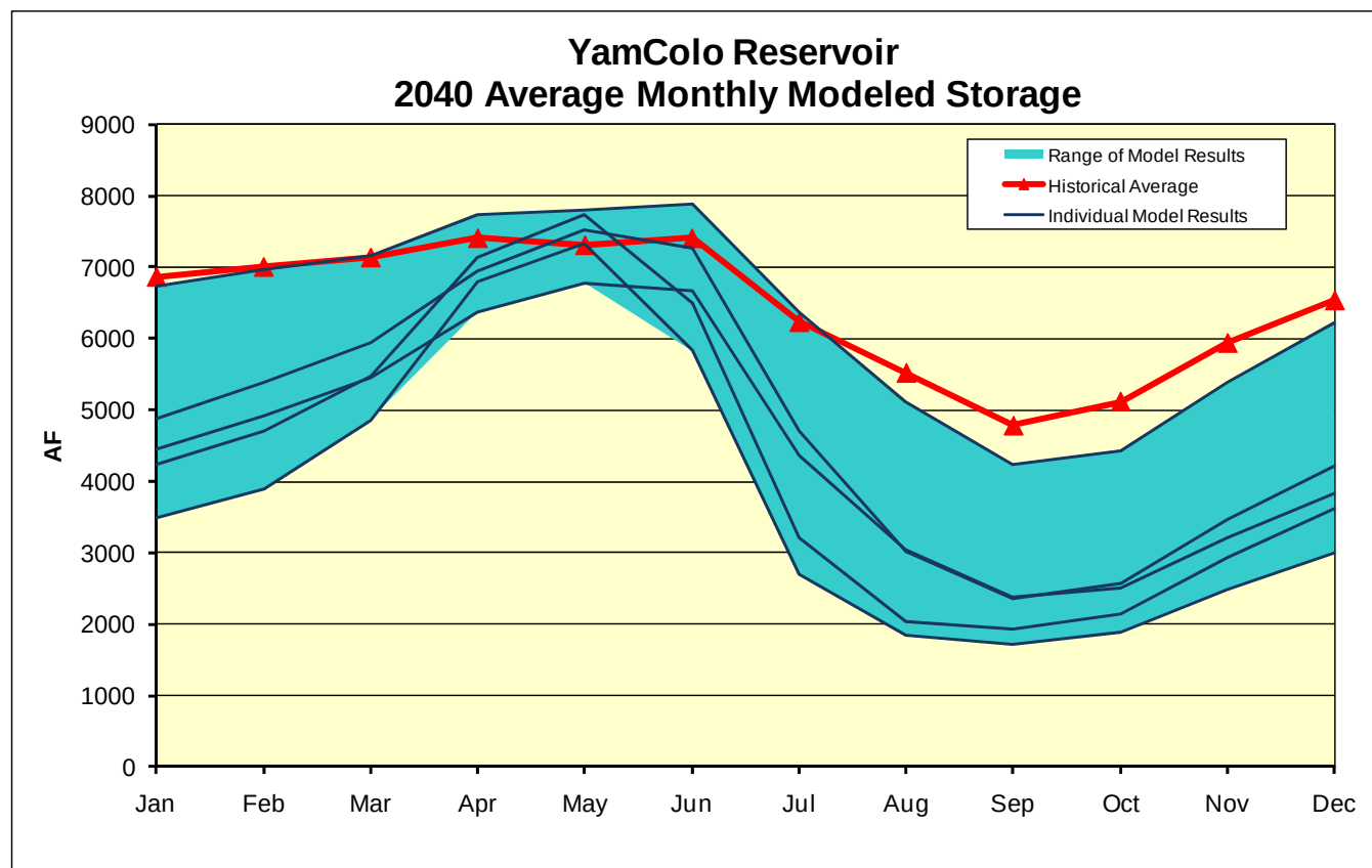
Figure 3-25 – Yamcolo Reservoir - 2040 Average Monthly Modeled Storage Content
