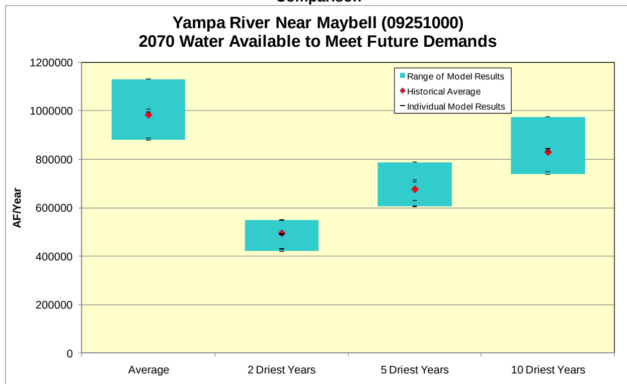
Figure F165 –2070 Yampa River near Maybell Water Available to Meet Future Demands Low-flow Comparison
