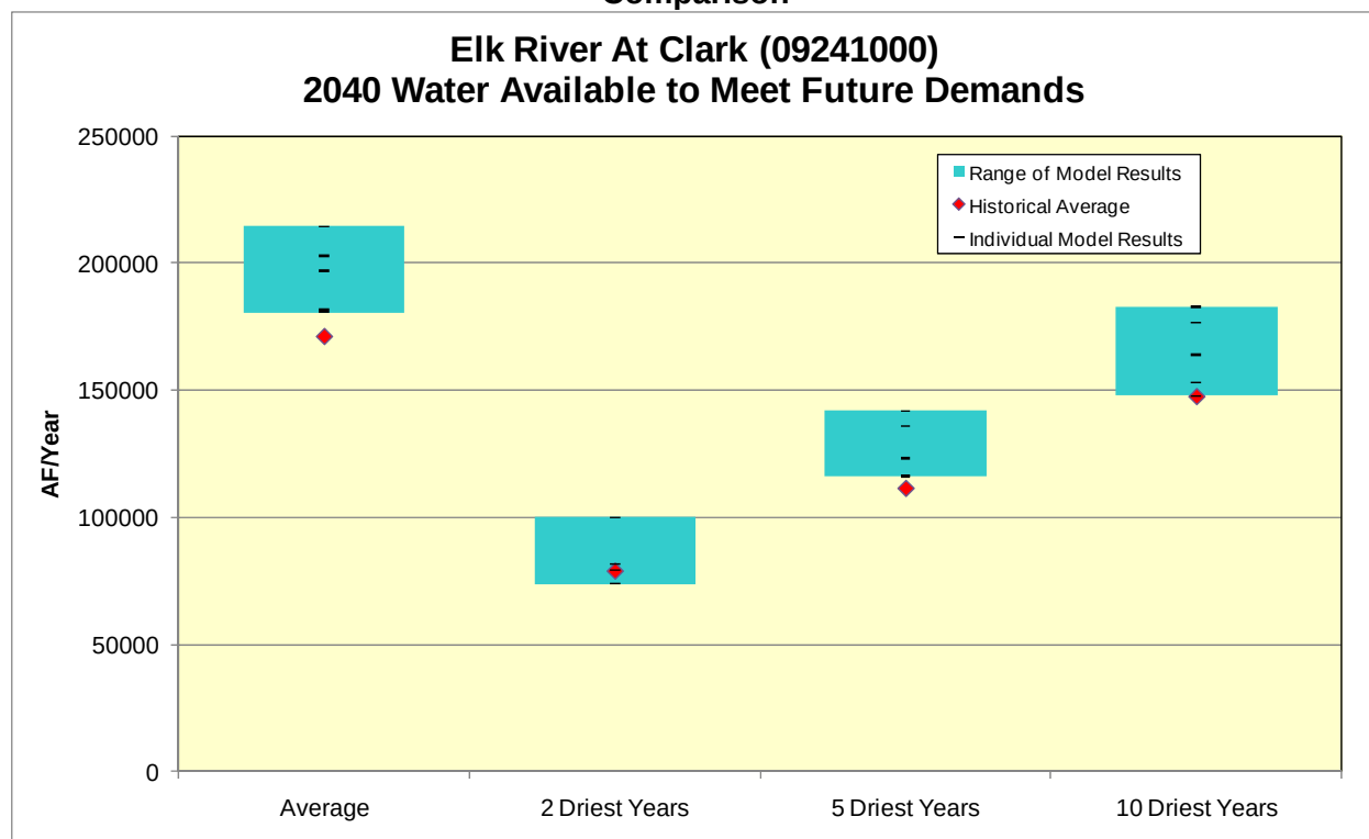
Figure F119 –2040 Elk River at Clark Water Available to Meet Future Demands Low-flow Comparison
