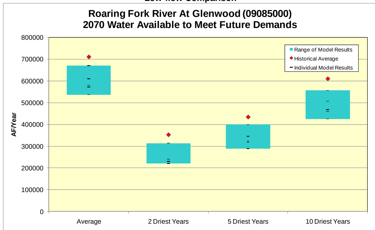
Figure F137 –2070 Roaring Fork River at Glenwood Water Available to Meet Future Demands Low-flow Comparison
