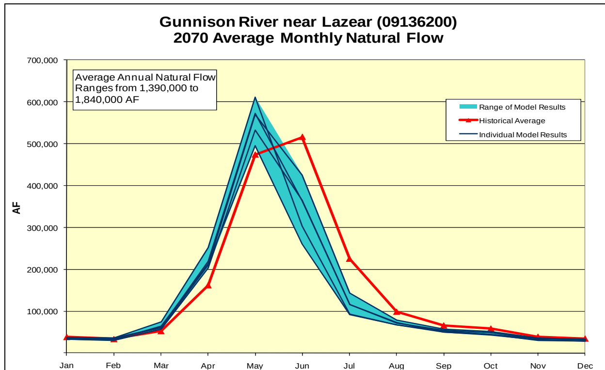
Figure D60 – 2070 Gunnison River near Lazez Average Monthly Natural Flow Comparison
