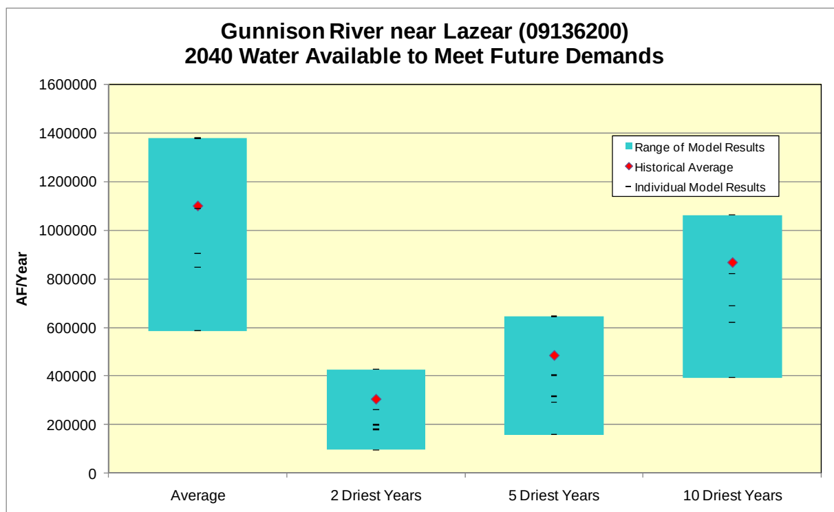
Figure F104 –2040 Gunnison River near Lazear Water Available to Meet Future Demands Low-flow Comparison
