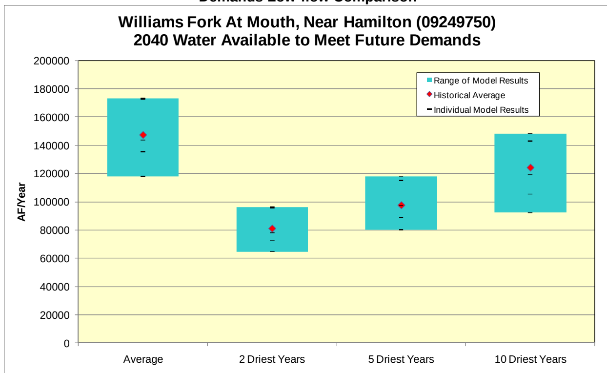
Figure F121 –2040 Williams Fork at Mouth, near Hamilton Water Available to Meet Future Demands Low-flow Comparison
