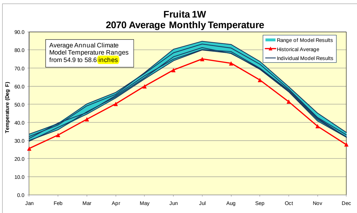
Figure A17 – Fruita 2070 Average Monthly Temperature Comparison
