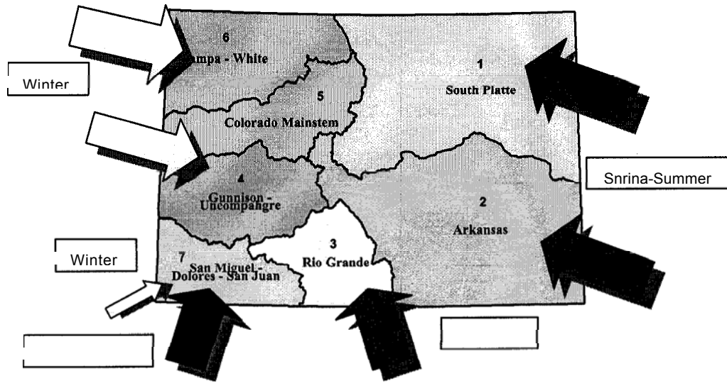
Sources of Atmospheric Moisture in Colorado Summer
