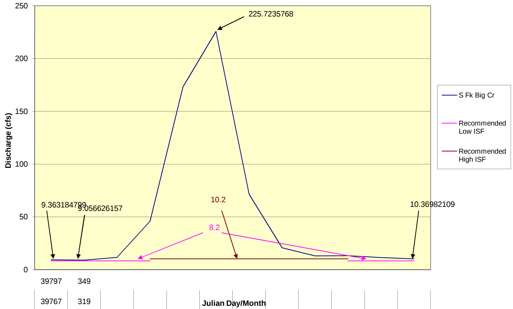
Figure 1 - Discharge S. Fk. Big Cr. (proportioned on Elk R. with irrigation consumption added back) and ISFs
