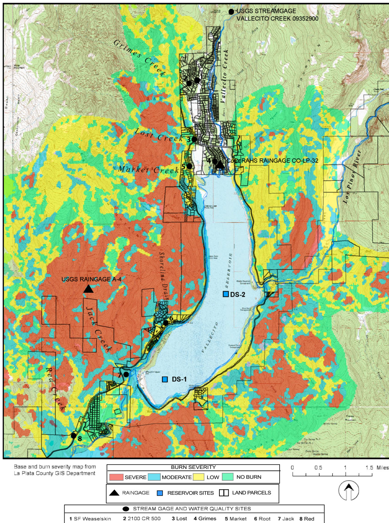
Figure 4. Site locations for measurement of rainfall, streamflow, and water-quality.
