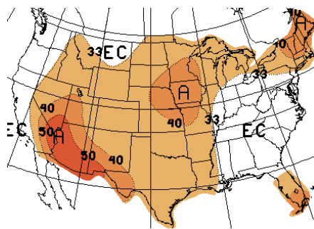
Figure 10d. Long-lead national temperature forecast for Sep. - Nov. 2006. (released June 15, 2006)
