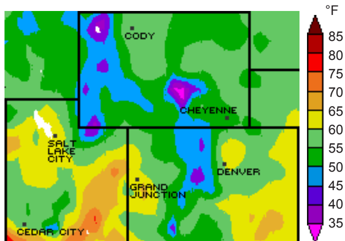
Figure 2a. Average temperature for the month of May 2006 in °F.
