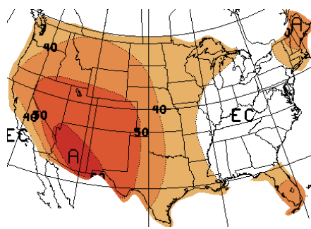
Figure 10b. Long-lead national temperature forecast for Jul. - Sep. 2006. (released June 15, 2006)
