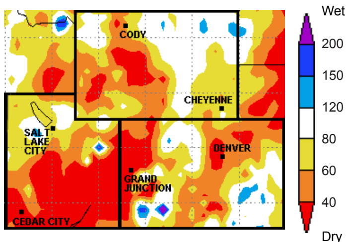
Figure 3b. Percent of average precipitation for the month of May 2006.
