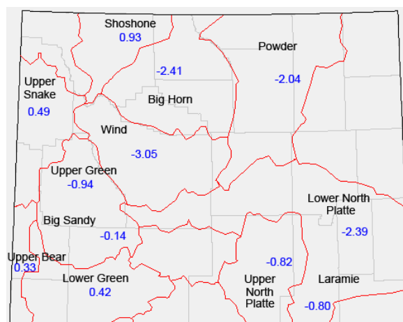
Figure 8b. Wyoming Surface Water Supply Index (data through 6/1/06)
