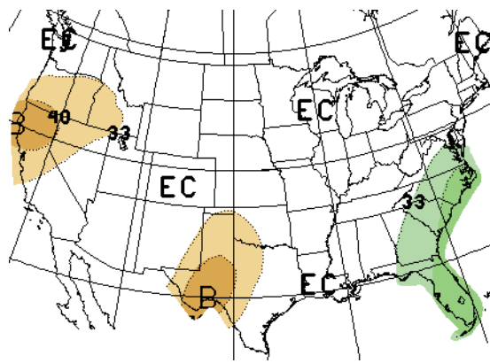
Figure 11b. Long-lead national precipitation forecast for Jun. - Aug. 2006. (released May 18, 2006)
