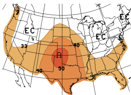
Figure 10a. Long-lead national temperature forecast for July 2006. (released June 15, 2006)
