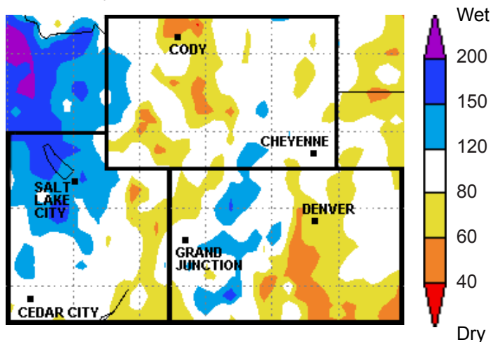
Figure 3c. Percent of average precipitation accumulated since the start of water year 2006. (Oct. 1 - May 30, 2006).
