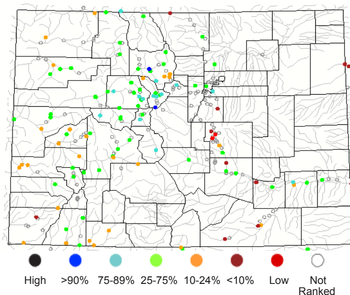
Figure 7b. Seven-day average streamflow conditions for points in Colorado as of 6/11/06.
