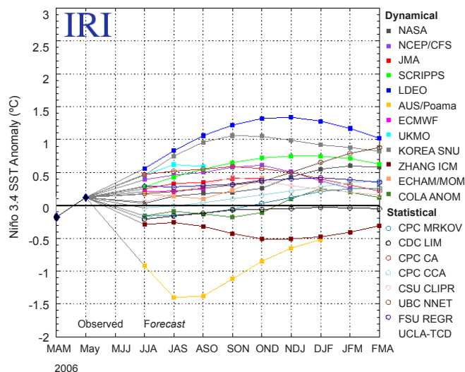
Figure 13b. Forecasts made by dynamical and statistical models for sea surface temperatures (SST) in the Niño 3.4 region for nine overlapping 3-month periods from June 2006 through April 2007 (released June, 13 2006). Forecasts are courtesy of the International Research Institute (IRI) for Climate and Society.
