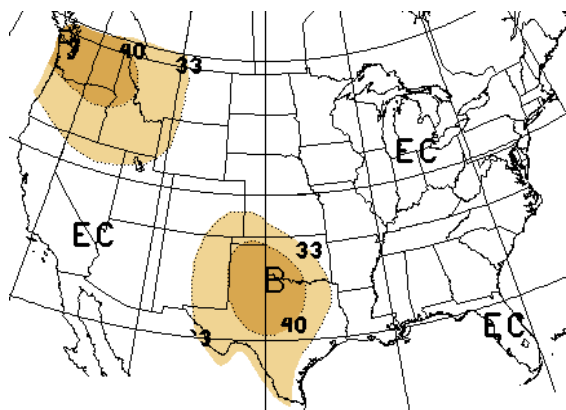
Figure 11a. Long-lead national precipitation forecast for June 2006. (released May 18, 2006)
