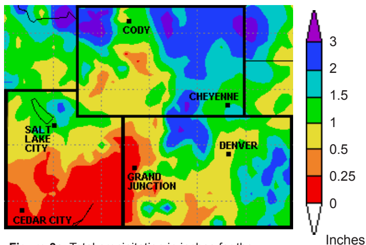
Figure 3a. Total precipitation in inches for the month of May 2006.
