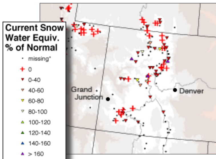
Figure 7a. Current snow water equivalent (SWE) as a percent of normal for SNOTEL sites in Colorado as of June 13, 2006. This is provisional data. For current SNOTEL data and plots of specific sites, see http://www.cbrfc.noaa.gov/snow/snow.cgi or http://www.wcc.nrcs.usda.gov/snow/ .
