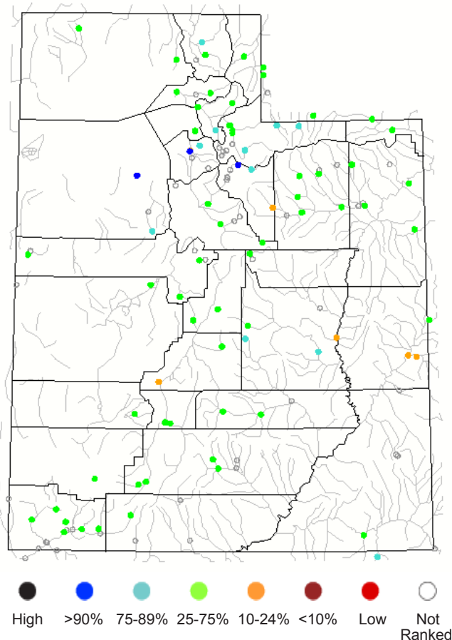
Figure 9b. Utah Percentile Streamflow Conditions (updated June 11, 2006).
