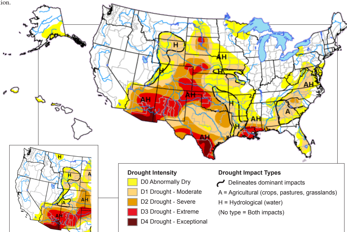
Figure 4. Drought Monitor released June 15, 2006 (full size) and last month May 16, 2006 (inset, lower left) for comparison.
