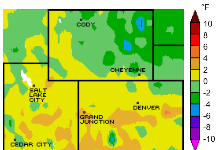
Figure 2c. Departure from average temperature in °F for last year, May 2005.
