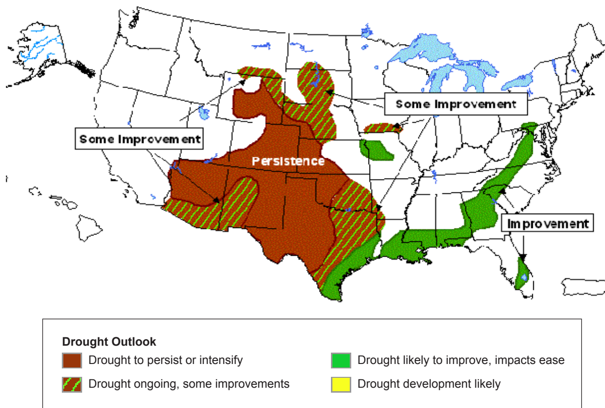
Figure 12. Seasonal Drought Outlook through September 2006 (release date June 15, 2006).
