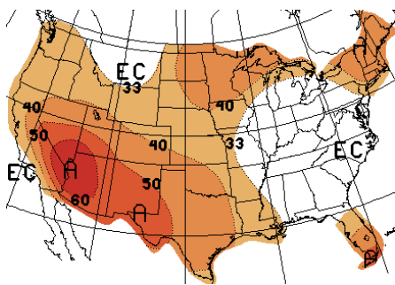
Figure 10c. Long-lead national temperature forecast for Aug. - Oct. 2006. (released June 15, 2006)
