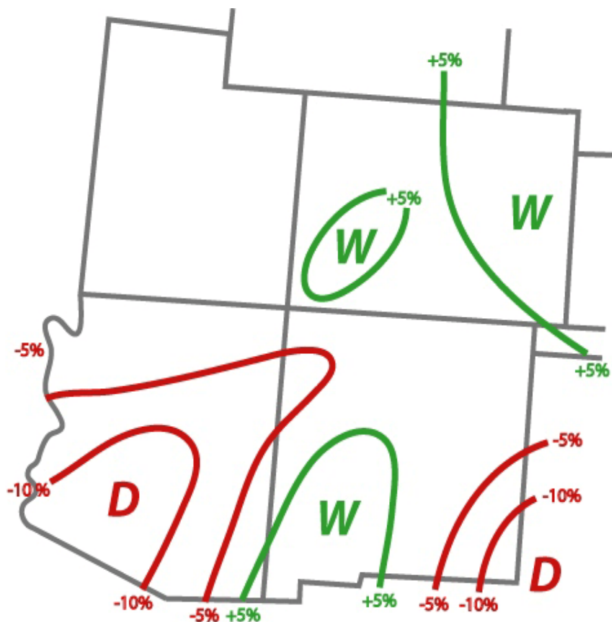
Figure 11c. Experimental guidance for seasonal precipitation in the southwest for July - September (issued June 14, 2006).
