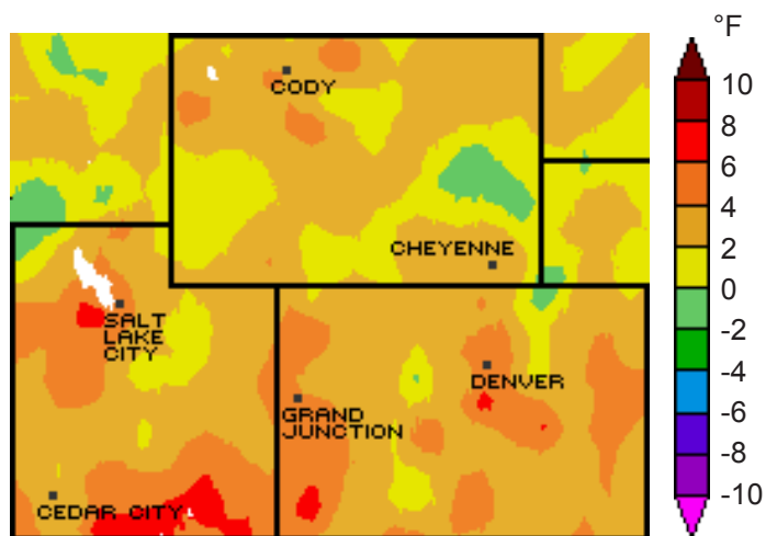
Figure 2b. Departure from average temperature for the month of May 2006 in °F.
