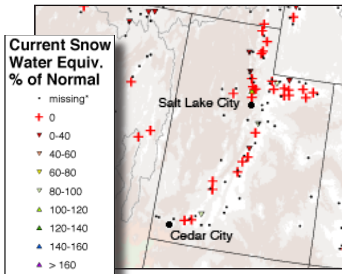
Figure 9a. Current snow water equivalent (SWE) as a percent of normal for SNOTEL sites in Utah as of June 13, 2006. This is provisional data. For current SNOTEL data and plots of specific sites, see http://www.cbafc.noaa.gov/snow/snow.cgi or http://www.wcc.nrcs.usda.gov/snow/
