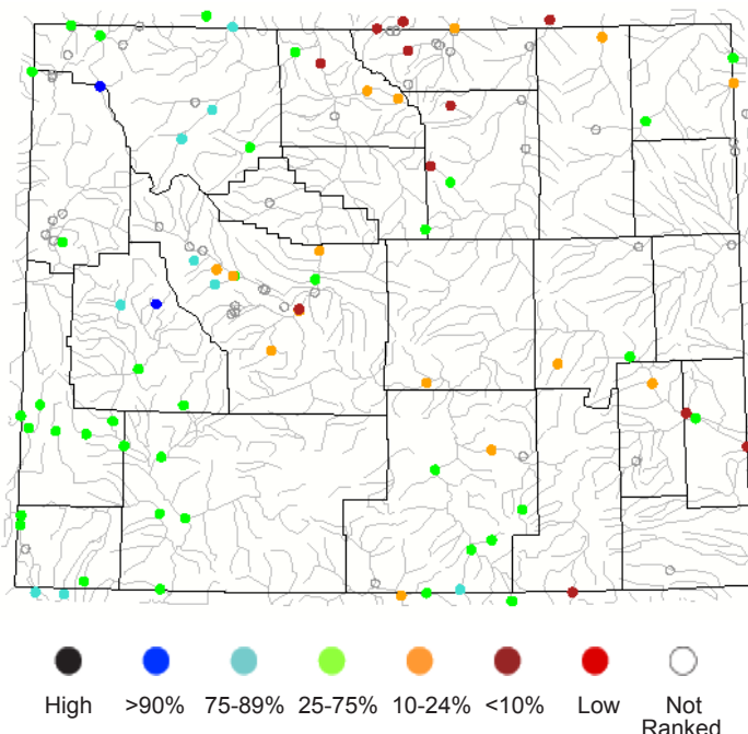
Figure 8a. Wyoming Percentile Streamflow Conditions (updated 6/11/06).
